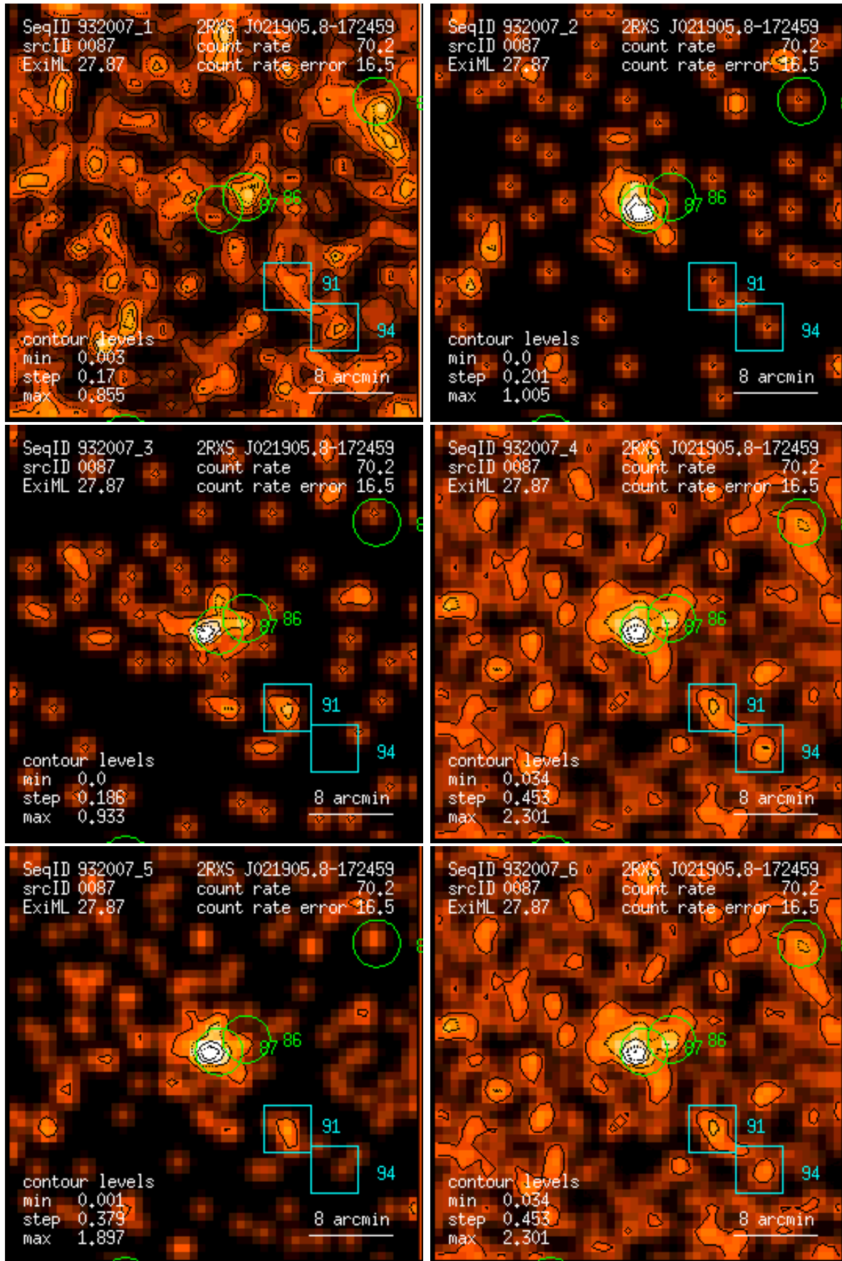
Figure 87: RASS 932007: detection 0087: band rate images, Gaussian filter: (1) PSPC channels 11 – 41, (2) 52 – 90, (3) 91 – 201, (4) 11 – 235, (5) 52 – 201, (6) 11 – 201. Broad band rates in counts/ks. Band rate contour levels in counts/ks/arcmin 2 .
