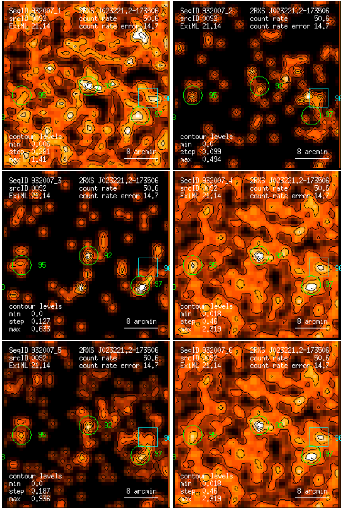
Figure 92: RASS 932007: detection 0092: band rate images, Gaussian filter: (1) PSPC channels 11 – 41, (2) 52 – 90, (3) 91 – 201, (4) 11 – 235, (5) 52 – 201, (6) 11 – 201. Broad band rates in counts/ks. Band rate contour levels in counts/ks/arcmin 2 .
