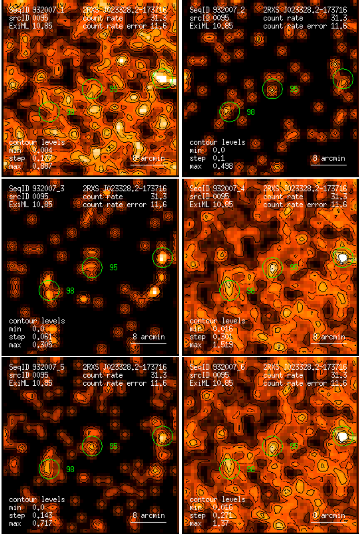
Figure 95: RASS 932007: detection 0095: band rate images, Gaussian filter: (1) PSPC channels 11 – 41, (2) 52 – 90, (3) 91 – 201, (4) 11 – 235, (5) 52 – 201, (6) 11 – 201. Broad band rates in counts/ks. Band rate contour levels in counts/ks/arcmin 2 .
