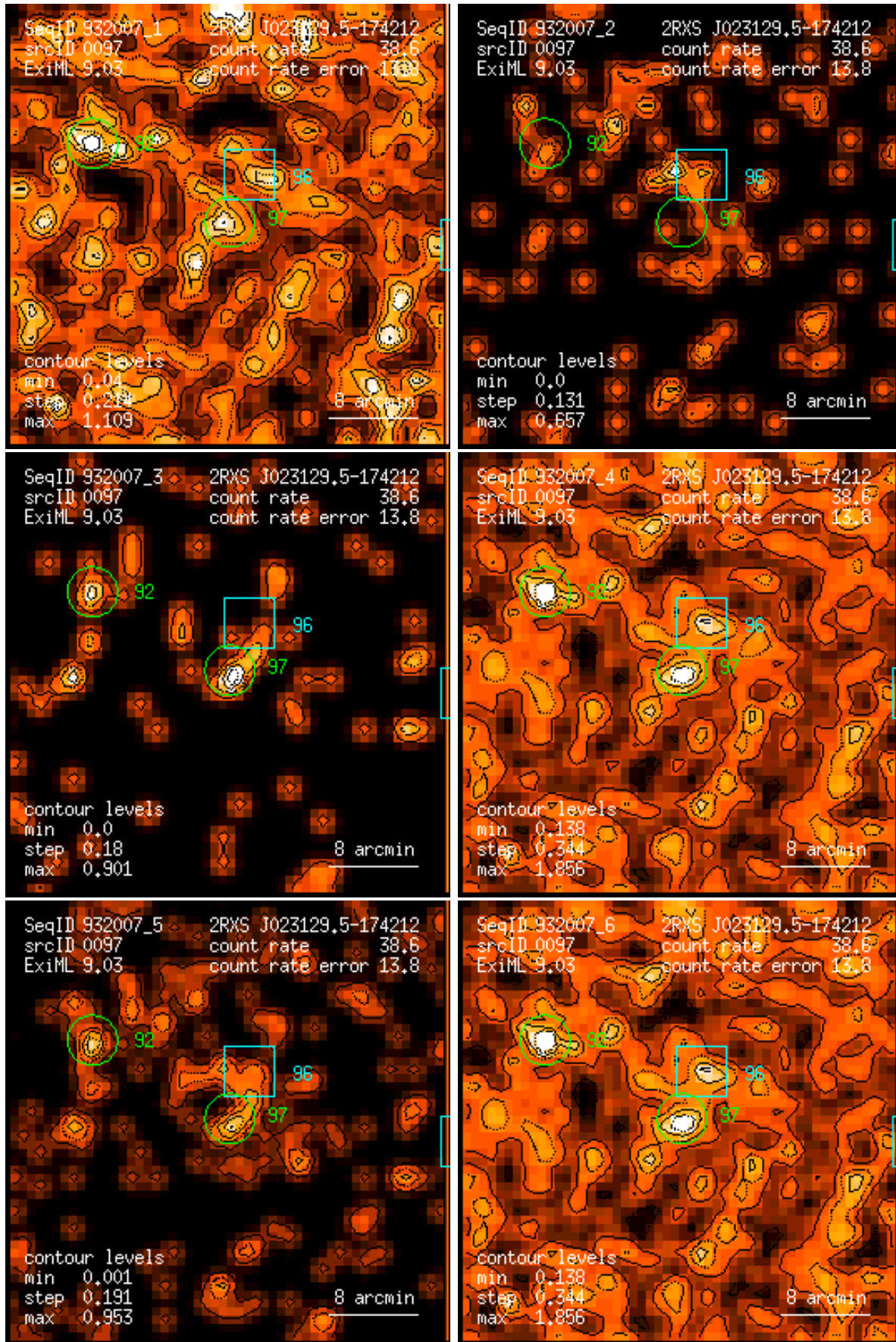
Figure 97: RASS 932007: detection 0097: band rate images, Gaussian filter: (1) PSPC channels 11 – 41, (2) 52 – 90, (3) 91 – 201, (4) 11 – 235, (5) 52 – 201, (6) 11 – 201. Broad band rates in counts/ks. Band rate contour levels in counts/ks/arcmin 2 .
