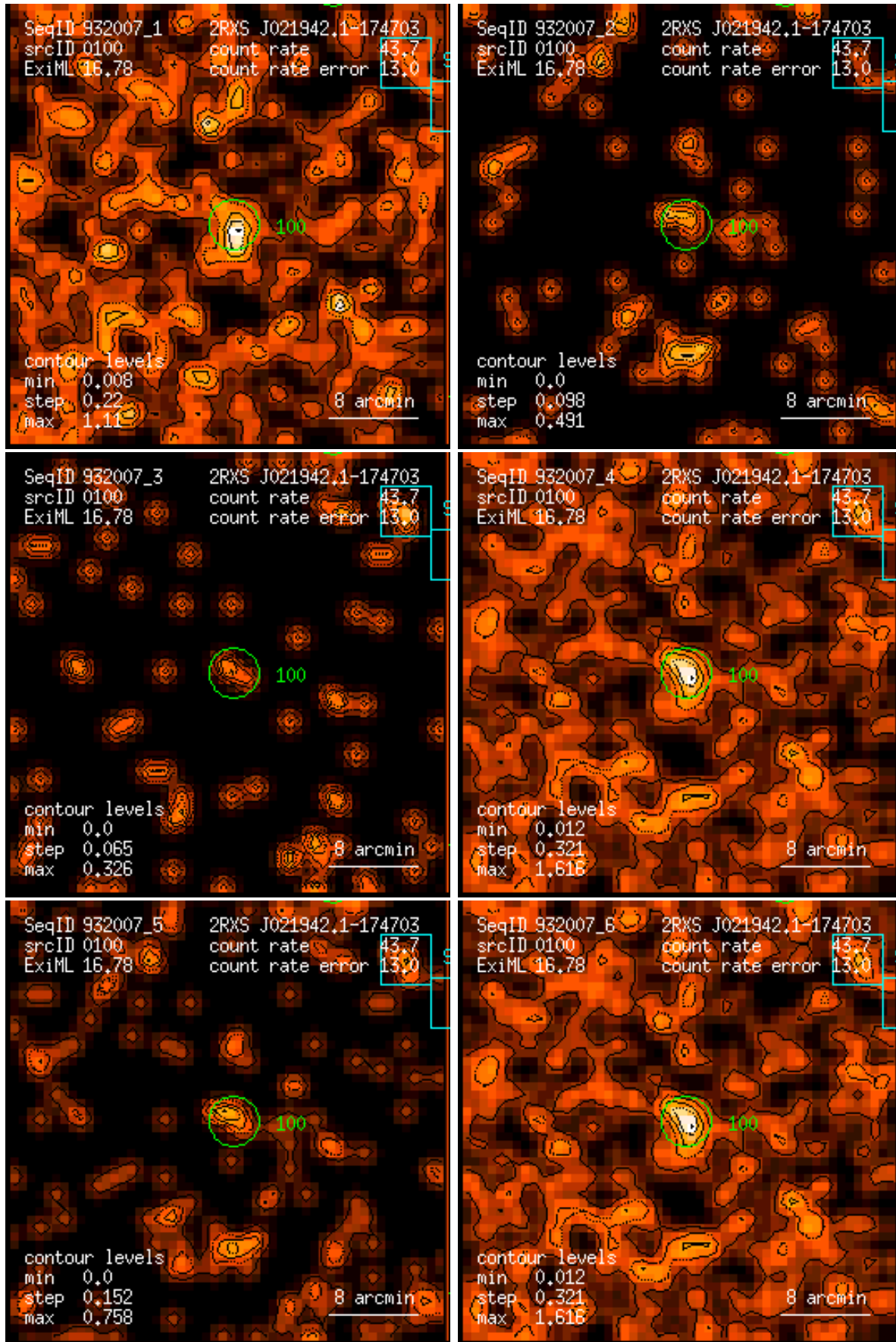
Figure 100: RASS 932007: detection 0100: band rate images, Gaussian filter: (1) PSPC channels 11 – 41, (2) 52 – 90, (3) 91 – 201, (4) 11 – 235, (5) 52 – 201, (6) 11 – 201. Broad band rates in counts/ks. Band rate contour levels in counts/ks/arcmin 2 .
