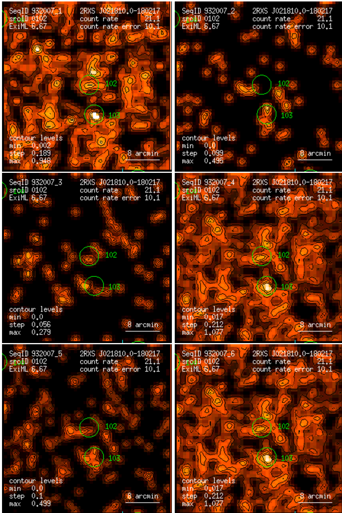
Figure 102: RASS 932007: detection 0102: band rate images, Gaussian filter: (1) PSPC channels 11 – 41, (2) 52 – 90, (3) 91 – 201, (4) 11 – 235, (5) 52 – 201, (6) 11 – 201. Broad band rates in counts/ks. Band rate contour levels in counts/ks/arcmin 2 .
