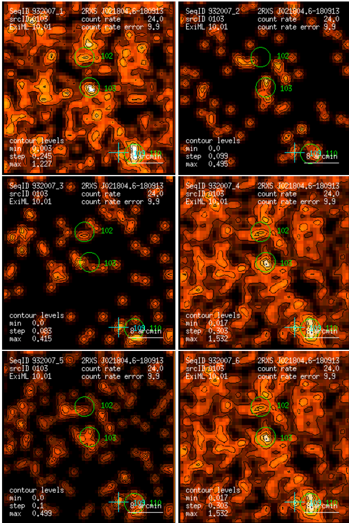
Figure 103: RASS 932007: detection 0103: band rate images, Gaussian filter: (1) PSPC channels 11 – 41, (2) 52 – 90, (3) 91 – 201, (4) 11 – 235, (5) 52 – 201, (6) 11 – 201. Broad band rates in counts/ks. Band rate contour levels in counts/ks/arcmin 2 .
