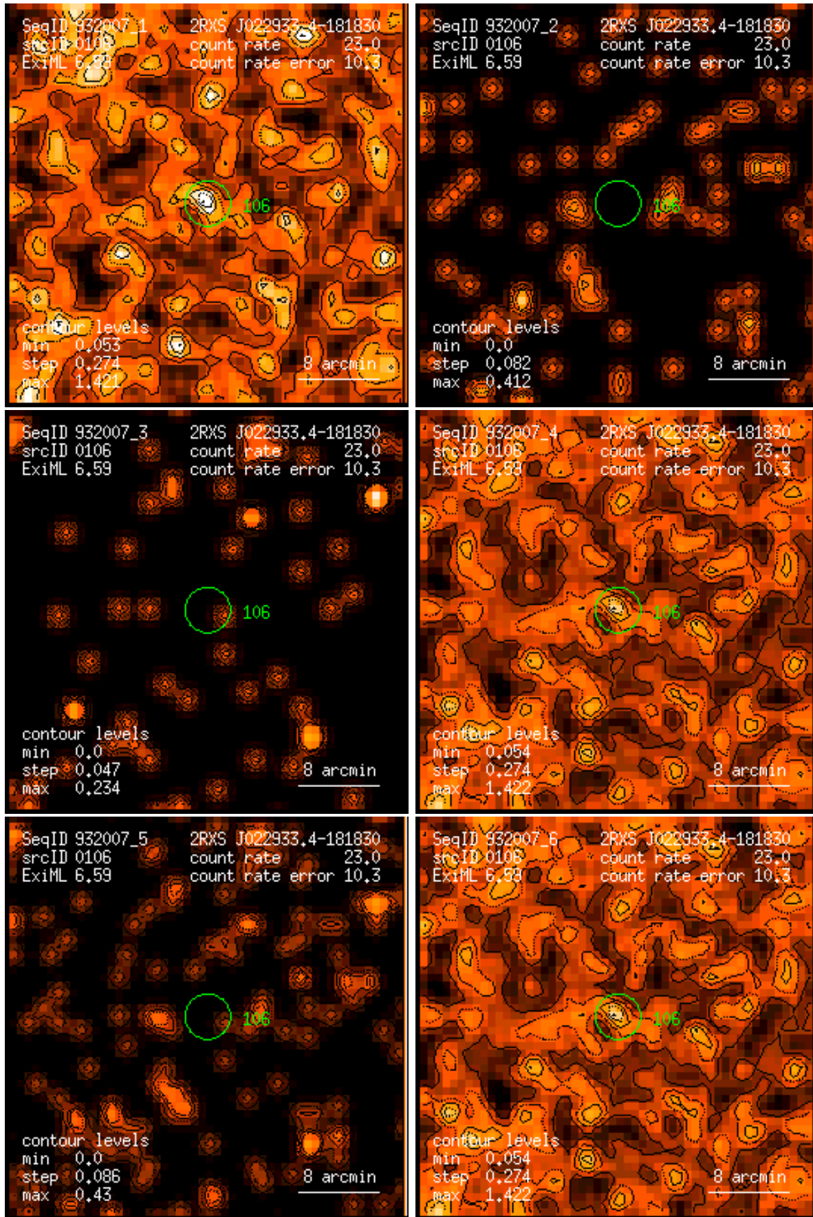
Figure 106: RASS 932007: detection 0106: band rate images, Gaussian filter: (1) PSPC channels 11 – 41, (2) 52 – 90, (3) 91 – 201, (4) 11 – 235, (5) 52 – 201, (6) 11 – 201. Broad band rates in counts/ks. Band rate contour levels in counts/ks/arcmin 2 .
