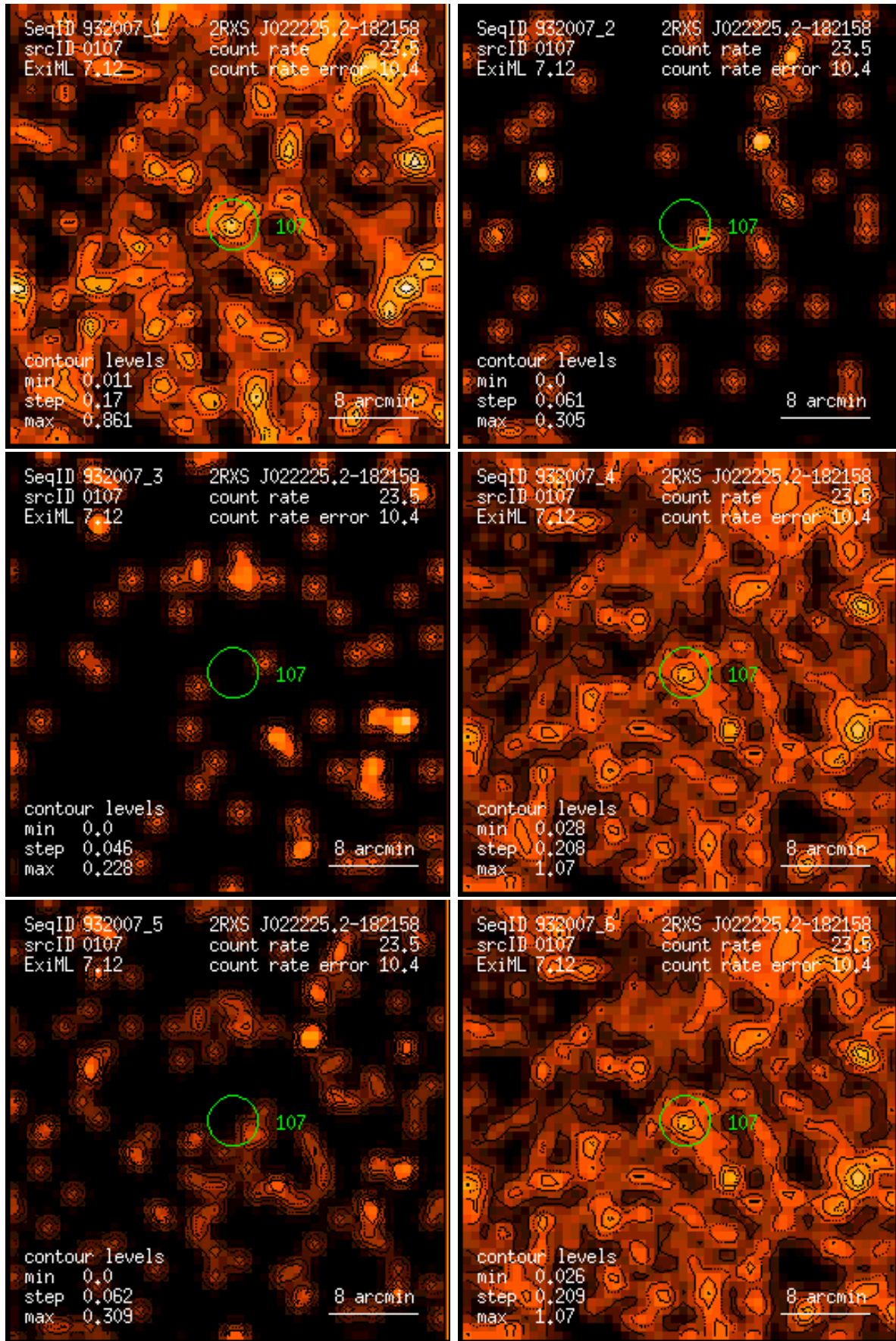
Figure 107: RASS 932007: detection 0107: band rate images, Gaussian filter: (1) PSPC channels 11 – 41, (2) 52 – 90, (3) 91 – 201, (4) 11 – 235, (5) 52 – 201, (6) 11 – 201. Broad band rates in counts/ks. Band rate contour levels in counts/ks/arcmin 2 .
