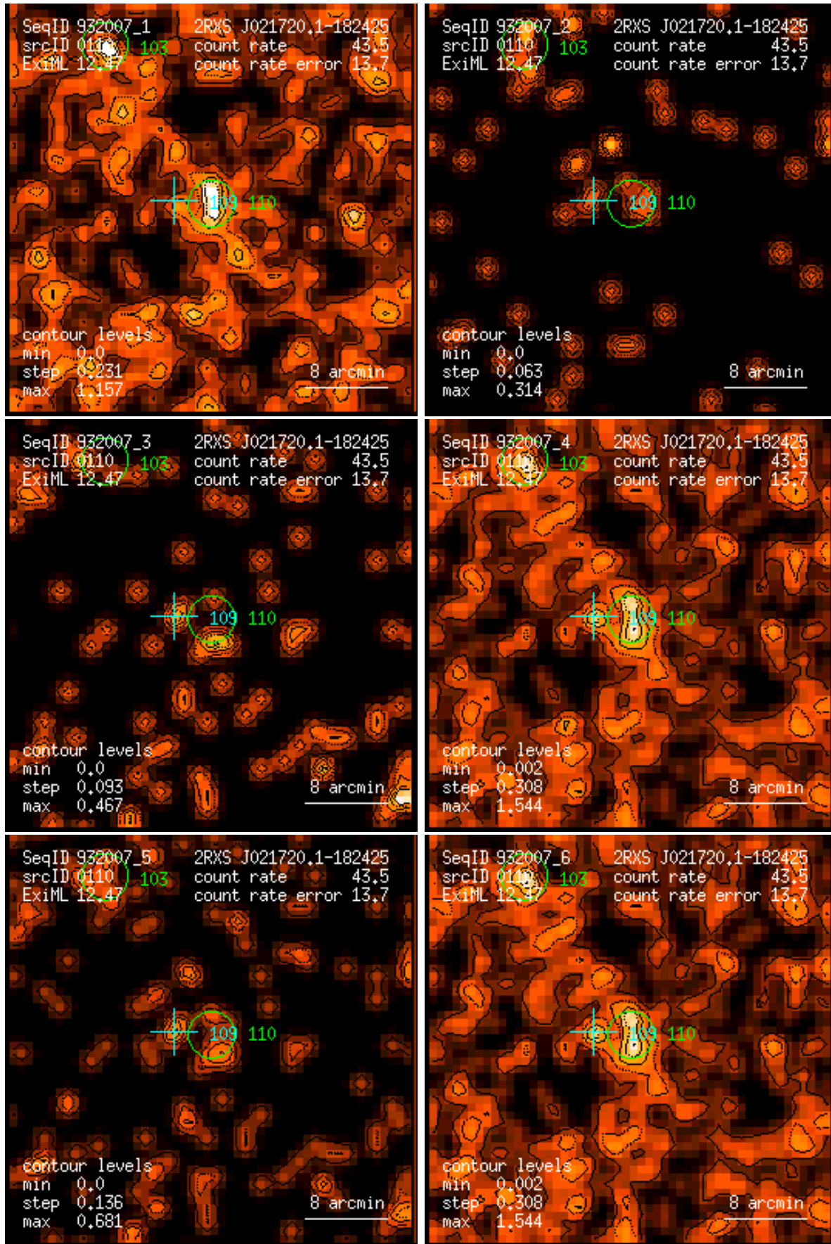
Figure 110: RASS 932007: detection 0110: band rate images, Gaussian filter: (1) PSPC channels 11 – 41, (2) 52 – 90, (3) 91 – 201, (4) 11 – 235, (5) 52 – 201, (6) 11 – 201. Broad band rates in counts/ks. Band rate contour levels in counts/ks/arcmin 2 .
