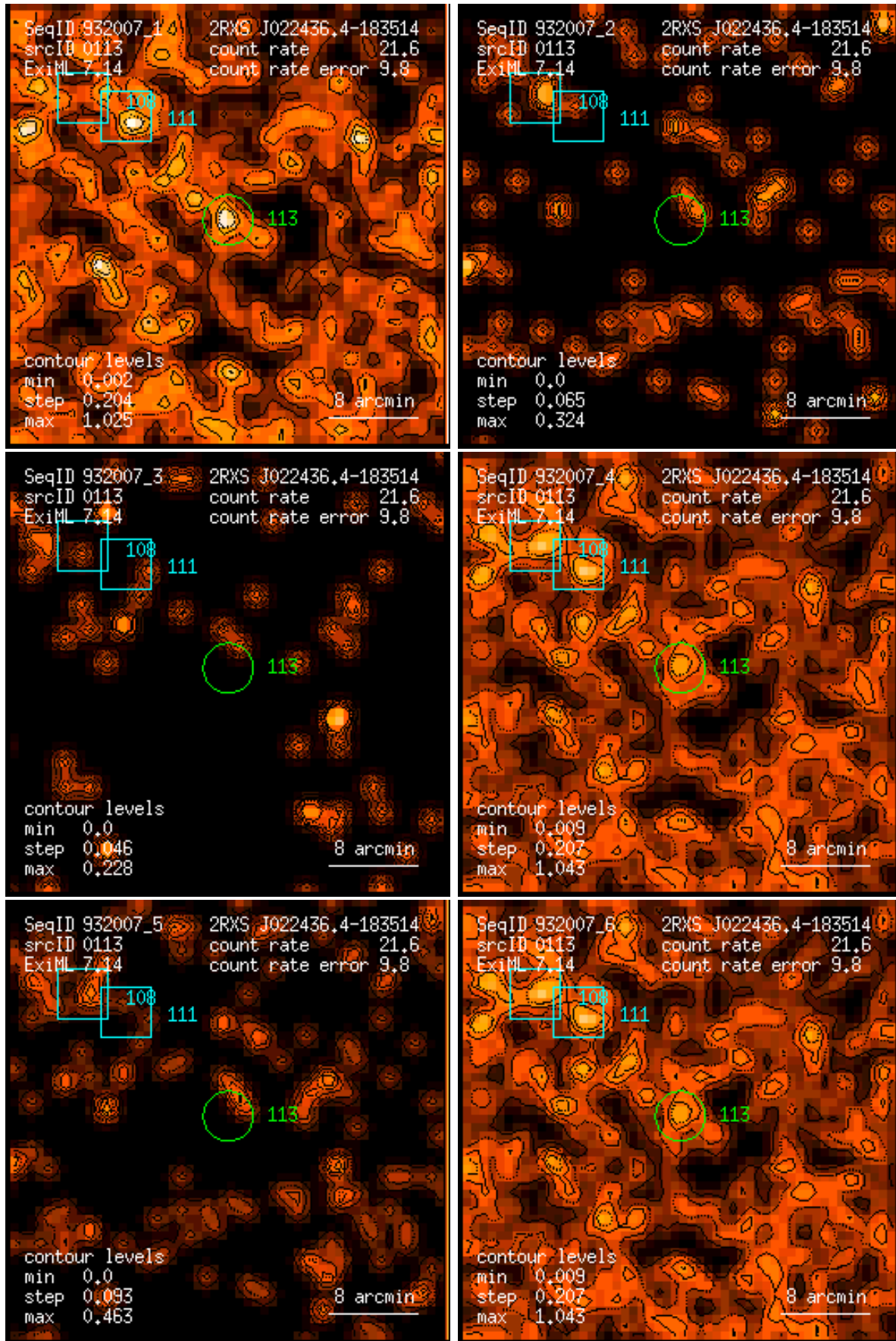
Figure 113: RASS 932007: detection 0113: band rate images, Gaussian filter: (1) PSPC channels 11 – 41, (2) 52 – 90, (3) 91 – 201, (4) 11 – 235, (5) 52 – 201, (6) 11 – 201. Broad band rates in counts/ks. Band rate contour levels in counts/ks/arcmin 2 .
