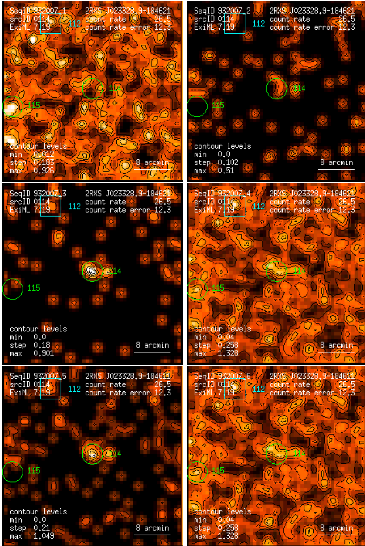
Figure 114: RASS 932007: detection 0114: band rate images, Gaussian filter: (1) PSPC channels 11 – 41, (2) 52 – 90, (3) 91 – 201, (4) 11 – 235, (5) 52 – 201, (6) 11 – 201. Broad band rates in counts/ks. Band rate contour levels in counts/ks/arcmin 2 .
