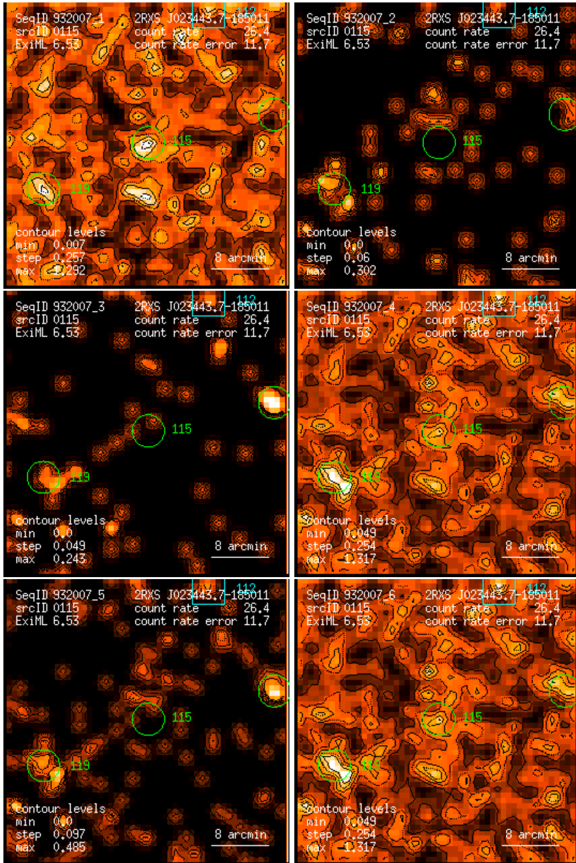
Figure 115: RASS 932007: detection 0115: band rate images, Gaussian filter: (1) PSPC channels 11 – 41, (2) 52 – 90, (3) 91 – 201, (4) 11 – 235, (5) 52 – 201, (6) 11 – 201. Broad band rates in counts/ks. Band rate contour levels in counts/ks/arcmin 2 .
