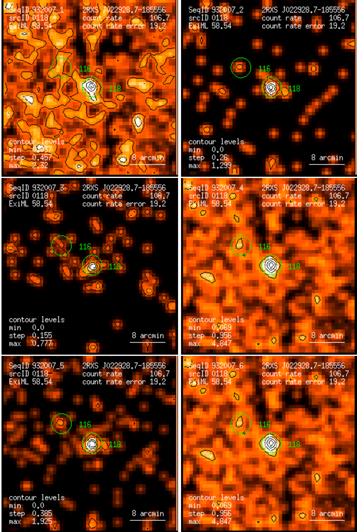
Figure 118: RASS 932007: detection 0118: band rate images, Gaussian filter: (1) PSPC channels 11 – 41, (2) 52 – 90, (3) 91 – 201, (4) 11 – 235, (5) 52 – 201, (6) 11 – 201. Broad band rates in counts/ks. Band rate contour levels in counts/ks/arcmin 2 .
