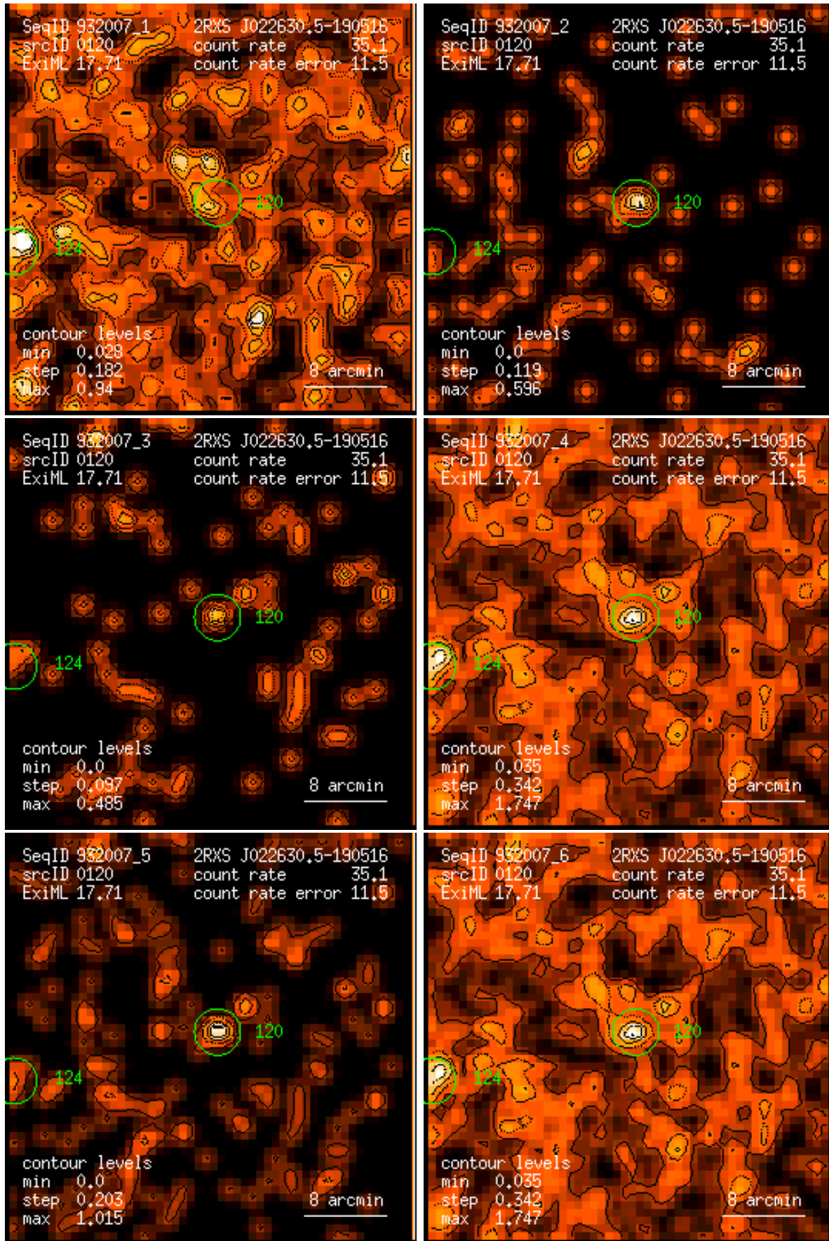
Figure 120: RASS 932007: detection 0120: band rate images, Gaussian filter: (1) PSPC channels 11 – 41, (2) 52 – 90, (3) 91 – 201, (4) 11 – 235, (5) 52 – 201, (6) 11 – 201. Broad band rates in counts/ks. Band rate contour levels in counts/ks/arcmin 2 .
