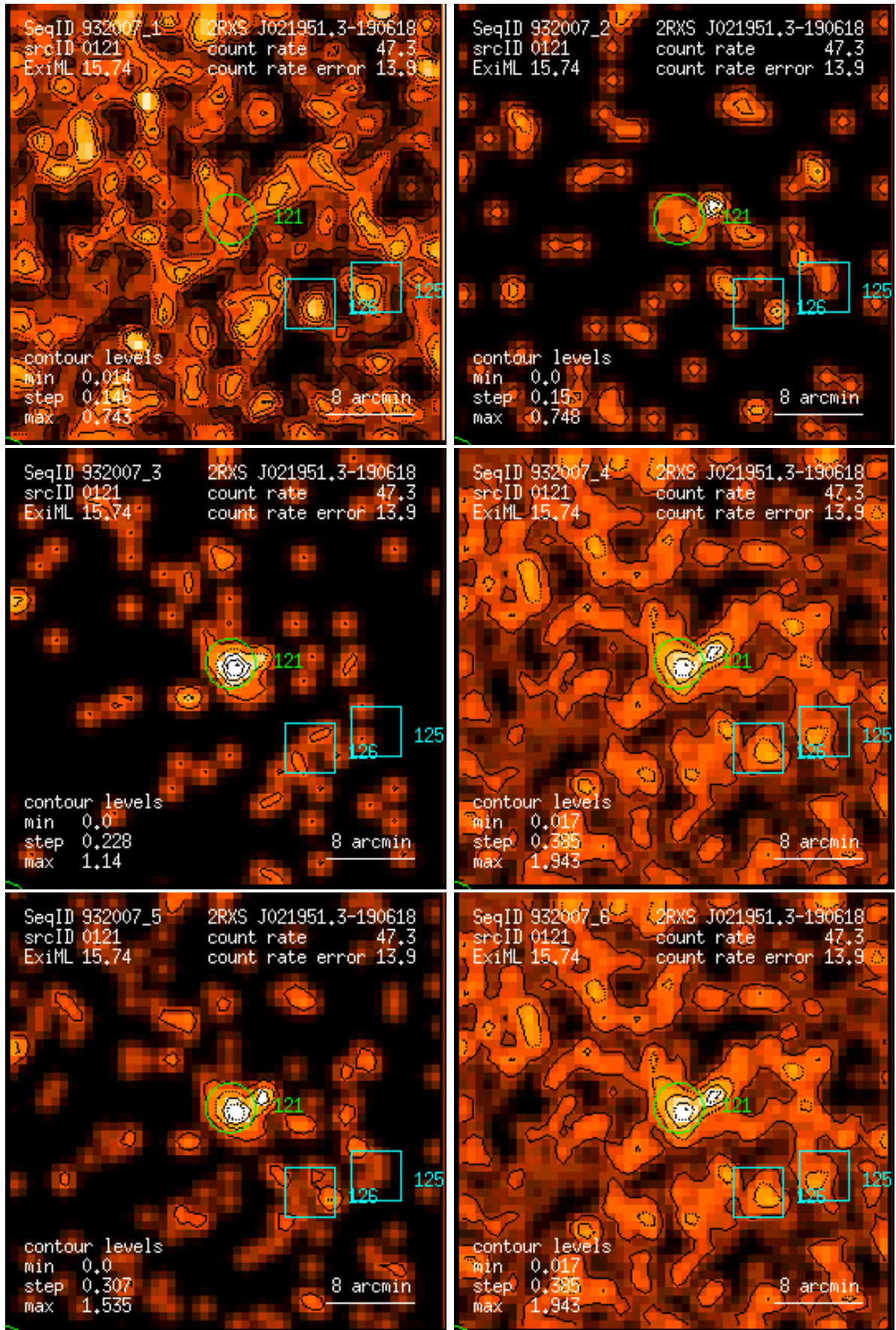
Figure 121: RASS 932007: detection 0121: band rate images, Gaussian filter: (1) PSPC channels 11 – 41, (2) 52 – 90, (3) 91 – 201, (4) 11 – 235, (5) 52 – 201, (6) 11 – 201. Broad band rates in counts/ks. Band rate contour levels in counts/ks/arcmin 2 .
