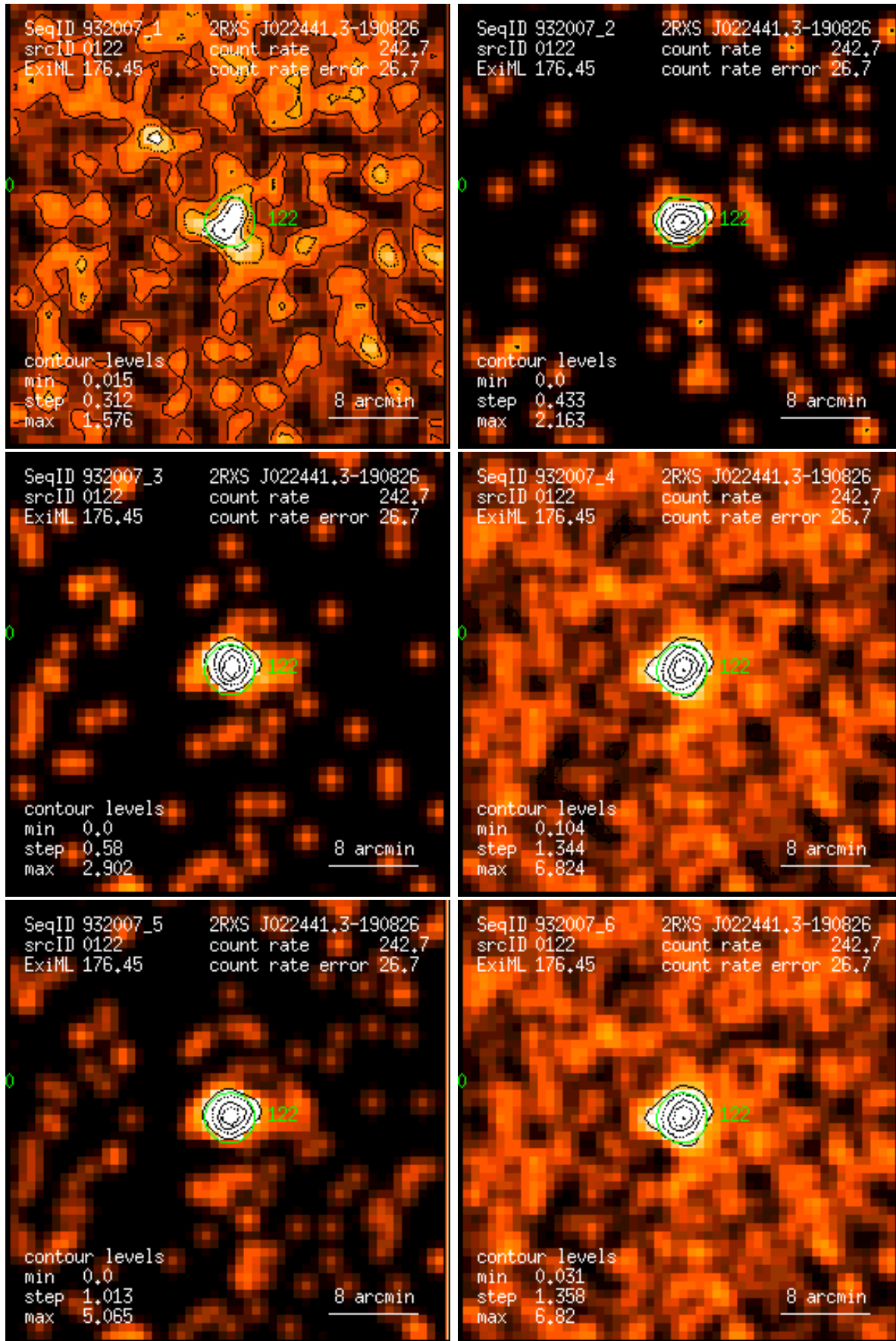
Figure 122: RASS 932007: detection 0122: band rate images, Gaussian filter: (1) PSPC channels 11 – 41, (2) 52 – 90, (3) 91 – 201, (4) 11 – 235, (5) 52 – 201, (6) 11 – 201. Broad band rates in counts/ks. Band rate contour levels in counts/ks/arcmin 2 .
