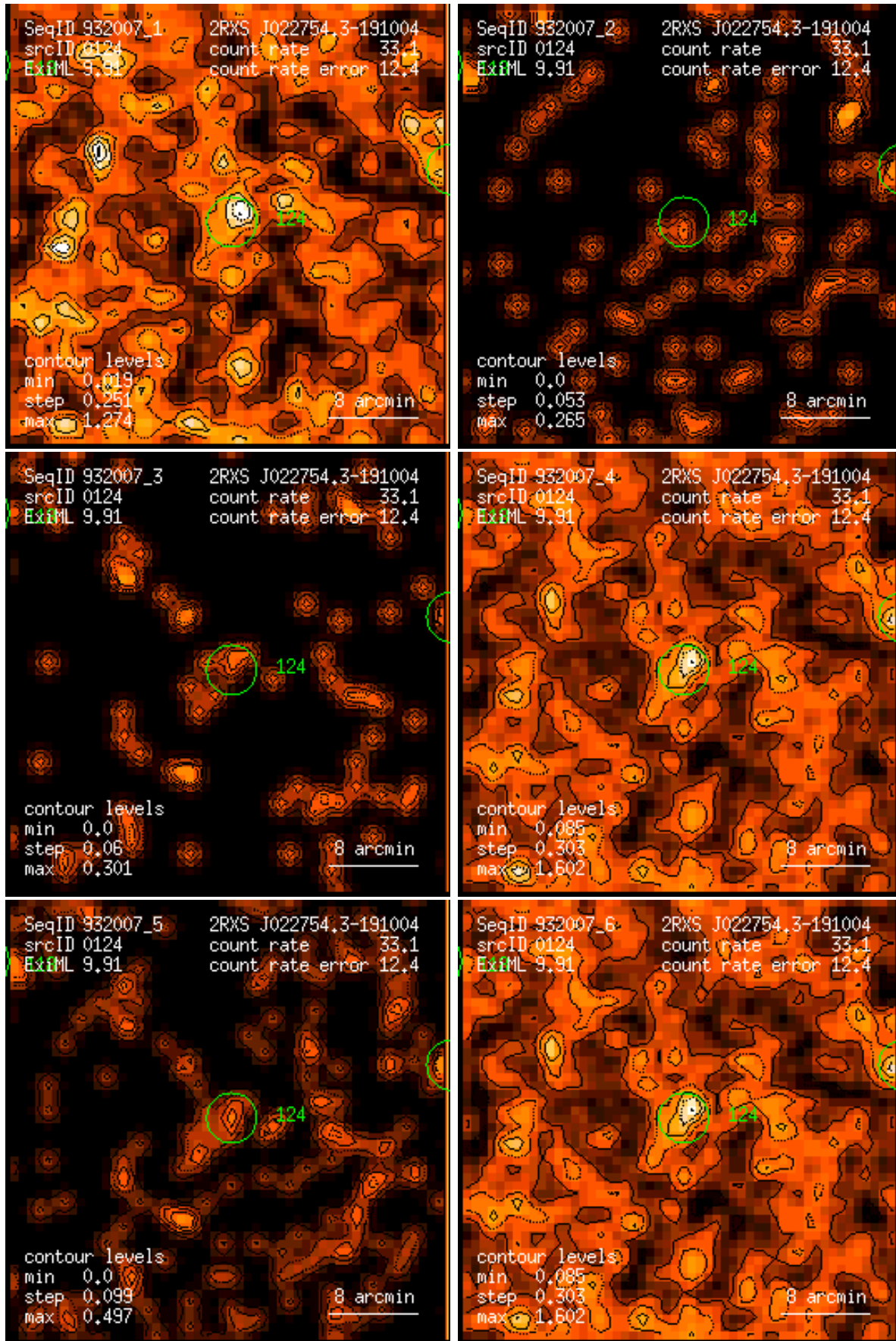
Figure 124: RASS 932007: detection 0124: band rate images, Gaussian filter: (1) PSPC channels 11 – 41, (2) 52 – 90, (3) 91 – 201, (4) 11 – 235, (5) 52 – 201, (6) 11 – 201. Broad band rates in counts/ks. Band rate contour levels in counts/ks/arcmin 2 .
