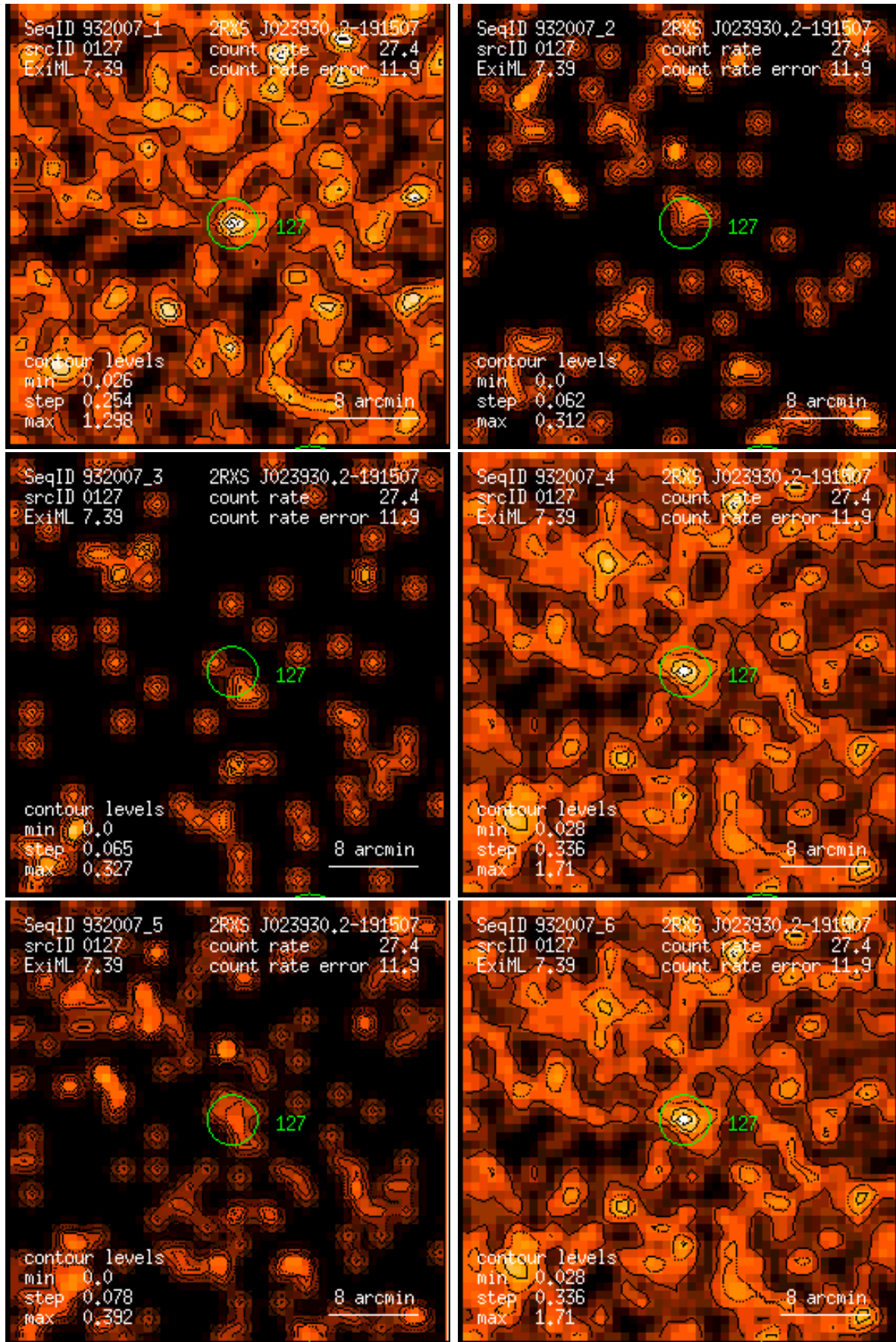
Figure 127: RASS 932007: detection 0127: band rate images, Gaussian filter: (1) PSPC channels 11 – 41, (2) 52 – 90, (3) 91 – 201, (4) 11 – 235, (5) 52 – 201, (6) 11 – 201. Broad band rates in counts/ks. Band rate contour levels in counts/ks/arcmin 2 .
