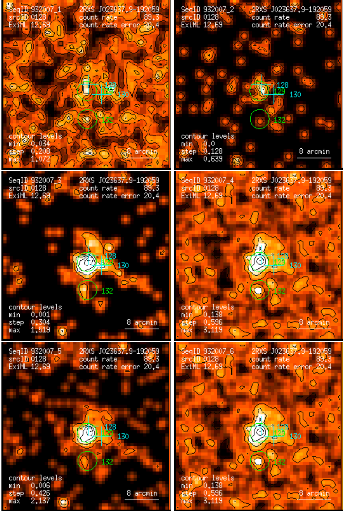
Figure 128: RASS 932007: detection 0128: band rate images, Gaussian filter: (1) PSPC channels 11 – 41, (2) 52 – 90, (3) 91 – 201, (4) 11 – 235, (5) 52 – 201, (6) 11 – 201. Broad band rates in counts/ks. Band rate contour levels in counts/ks/arcmin 2 .
