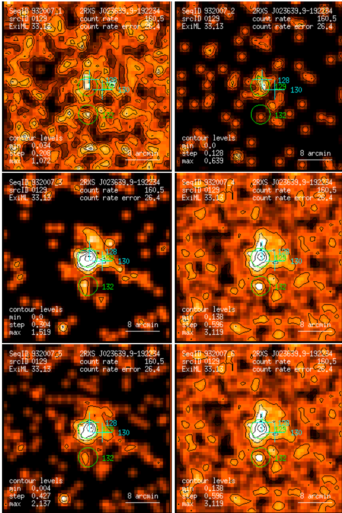
Figure 129: RASS 932007: detection 0129: band rate images, Gaussian filter: (1) PSPC channels 11 – 41, (2) 52 – 90, (3) 91 – 201, (4) 11 – 235, (5) 52 – 201, (6) 11 – 201. Broad band rates in counts/ks. Band rate contour levels in counts/ks/arcmin 2 .
