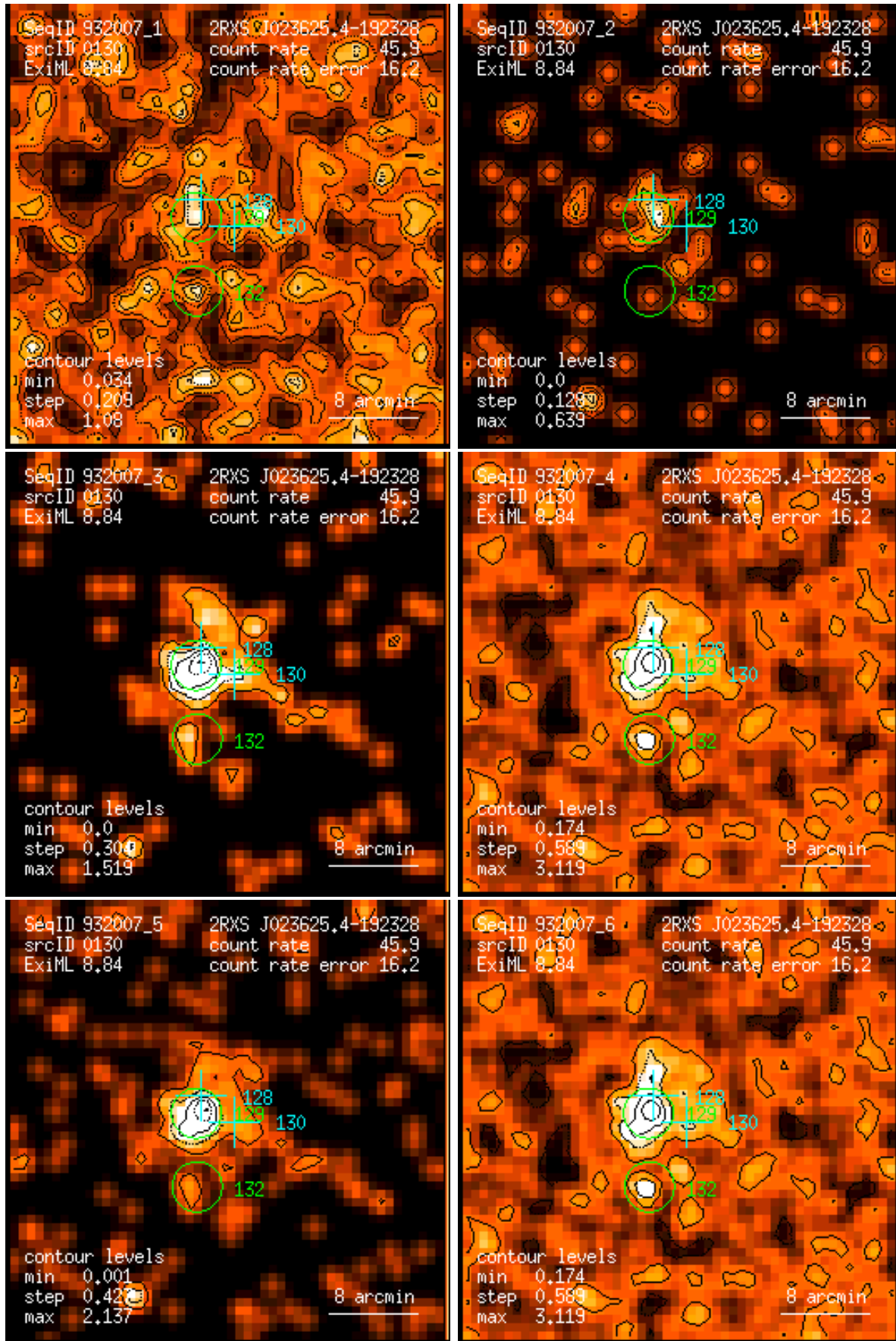
Figure 130: RASS 932007: detection 0130: band rate images, Gaussian filter: (1) PSPC channels 11 – 41, (2) 52 – 90, (3) 91 – 201, (4) 11 – 235, (5) 52 – 201, (6) 11 – 201. Broad band rates in counts/ks. Band rate contour levels in counts/ks/arcmin 2 .
