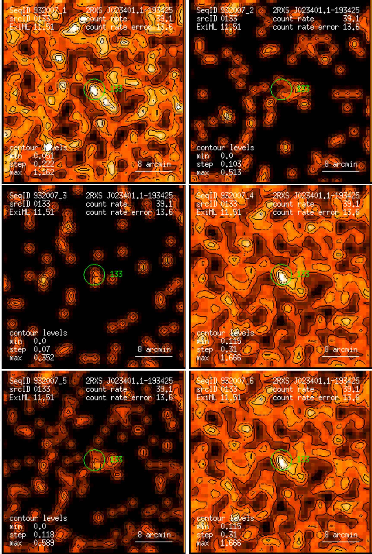
Figure 133: RASS 932007: detection 0133: band rate images, Gaussian filter: (1) PSPC channels 11 – 41, (2) 52 – 90, (3) 91 – 201, (4) 11 – 235, (5) 52 – 201, (6) 11 – 201. Broad band rates in counts/ks. Band rate contour levels in counts/ks/arcmin 2 .
