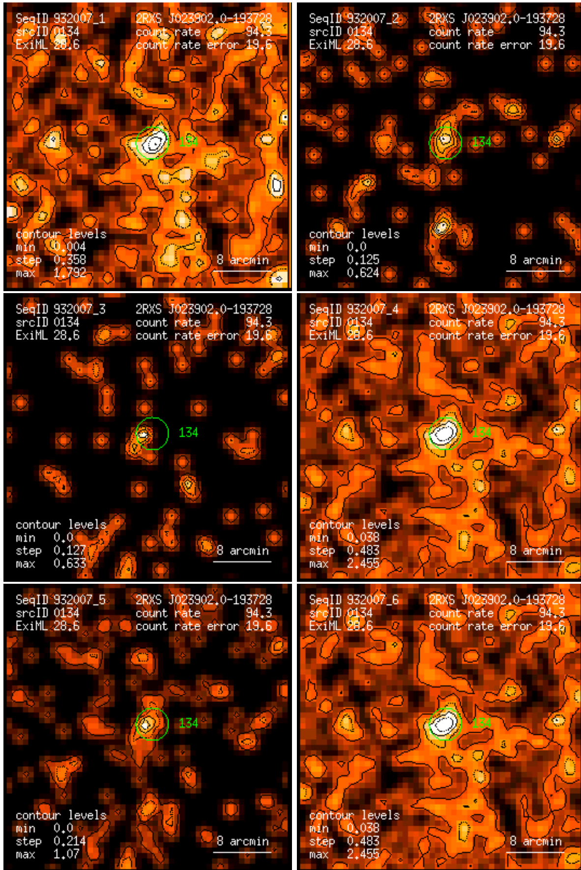
Figure 134: RASS 932007: detection 0134: band rate images, Gaussian filter: (1) PSPC channels 11 – 41, (2) 52 – 90, (3) 91 – 201, (4) 11 – 235, (5) 52 – 201, (6) 11 – 201. Broad band rates in counts/ks. Band rate contour levels in counts/ks/arcmin 2 .
