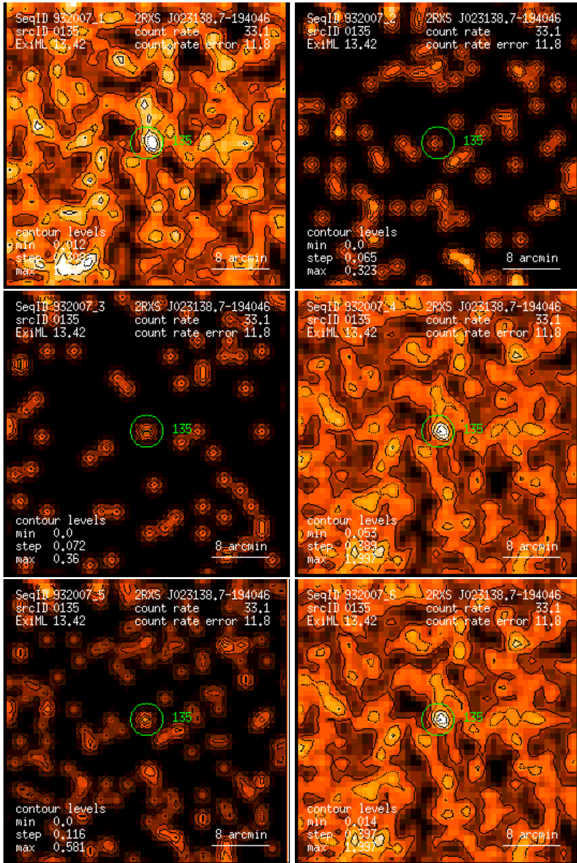
Figure 135: RASS 932007: detection 0135: band rate images, Gaussian filter: (1) PSPC channels 11 – 41, (2) 52 – 90, (3) 91 – 201, (4) 11 – 235, (5) 52 – 201, (6) 11 – 201. Broad band rates in counts/ks. Band rate contour levels in counts/ks/arcmin 2 .
