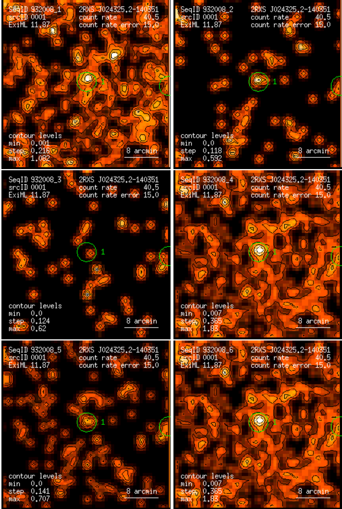
Figure 1: RASS 932008: detection 0001: band rate images, Gaussian filter: (1) PSPC channels 11 – 41, (2) 52 – 90, (3) 91 – 201, (4) 11 – 235, (5) 52 – 201, (6) 11 – 201. Broad band rates in counts/ks. Band rate contour levels in counts/ks/arcmin 2 .
