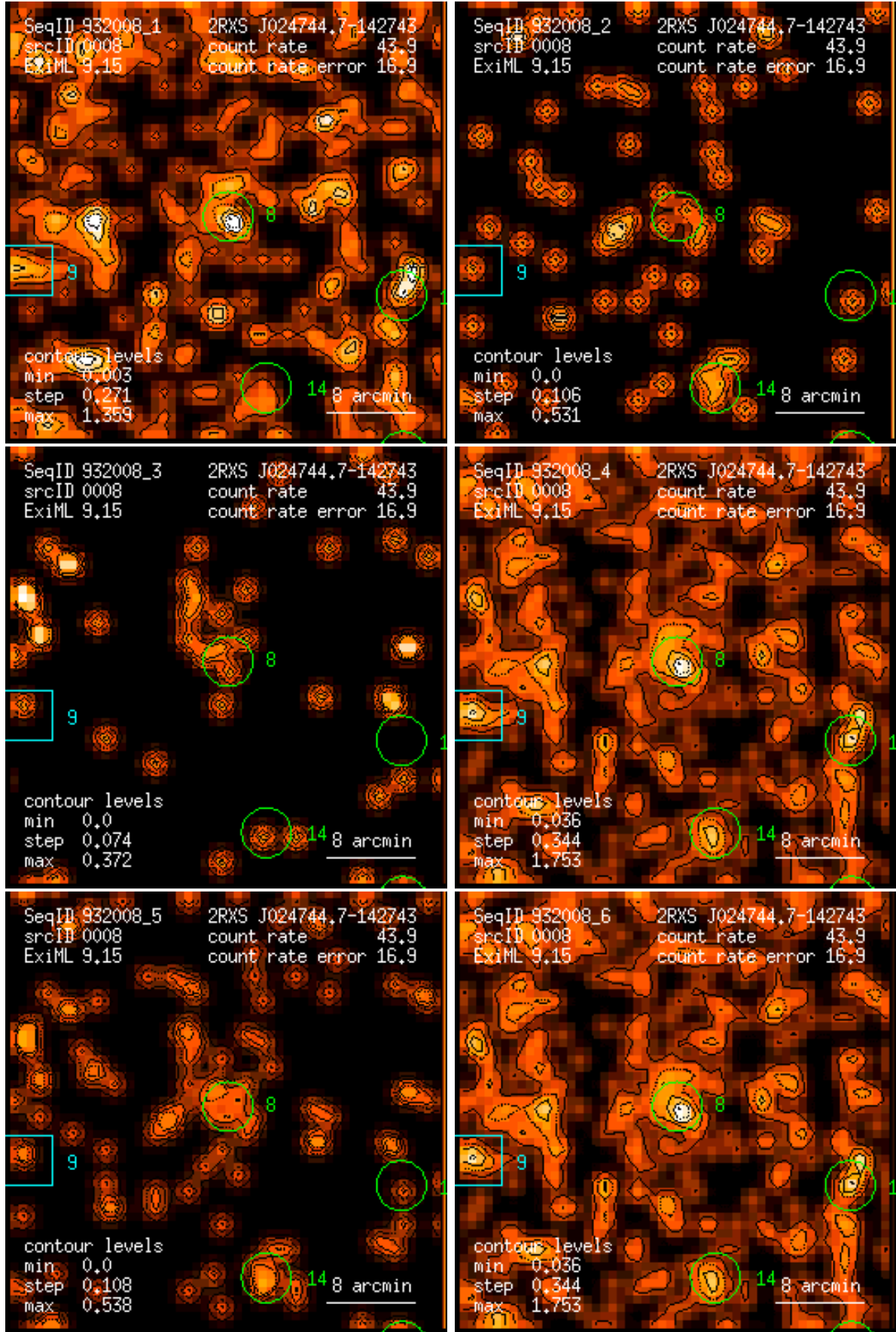
Figure 8: RASS 932008: detection 0008: band rate images, Gaussian filter: (1) PSPC channels 11 – 41, (2) 52 – 90, (3) 91 – 201, (4) 11 – 235, (5) 52 – 201, (6) 11 – 201. Broad band rates in counts/ks. Band rate contour levels in counts/ks/arcmin 2 .
