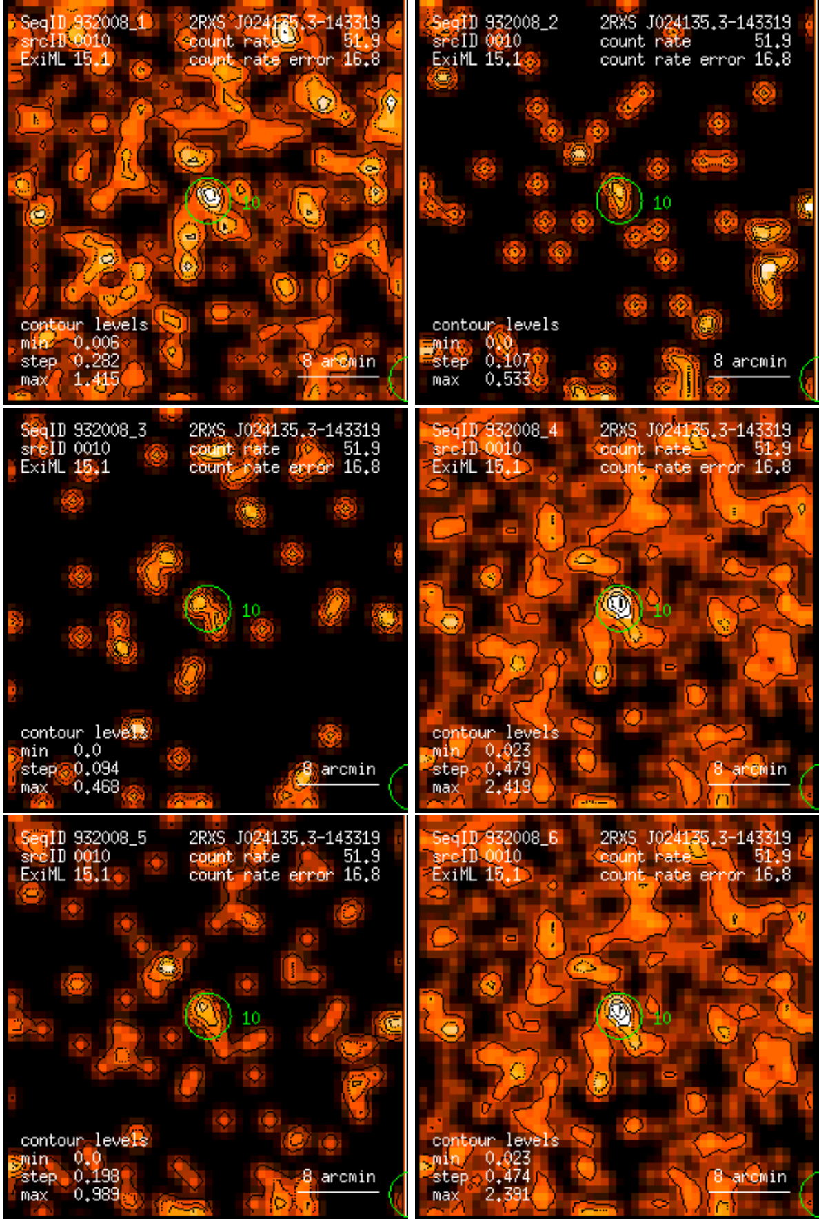
Figure 10: RASS 932008: detection 0010: band rate images, Gaussian filter: (1) PSPC channels 11 – 41, (2) 52 – 90, (3) 91 – 201, (4) 11 – 235, (5) 52 – 201, (6) 11 – 201. Broad band rates in counts/ks. Band rate contour levels in counts/ks/arcmin 2 .
