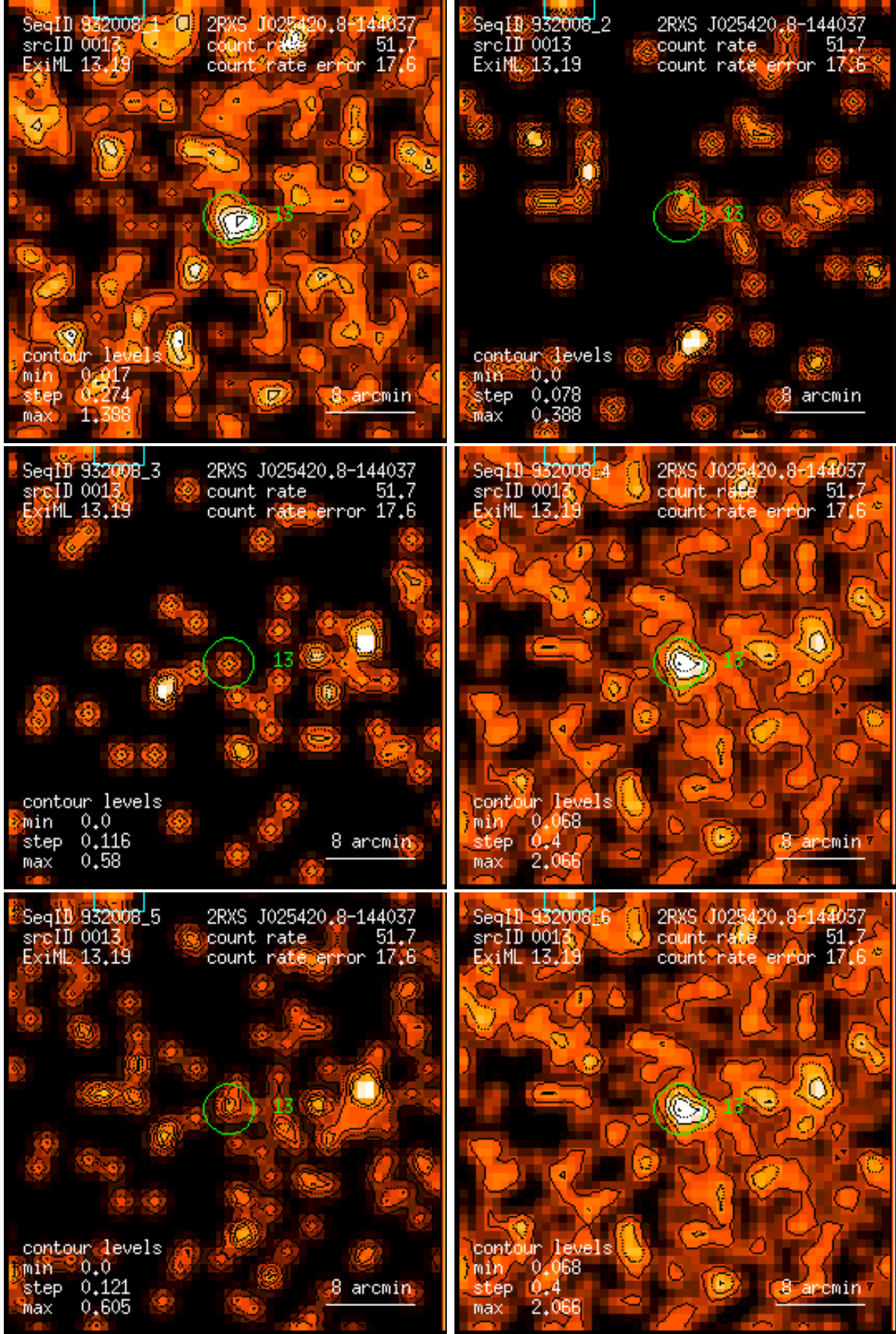
Figure 13: RASS 932008: detection 0013: band rate images, Gaussian filter: (1) PSPC channels 11 – 41, (2) 52 – 90, (3) 91 – 201, (4) 11 – 235, (5) 52 – 201, (6) 11 – 201. Broad band rates in counts/ks. Band rate contour levels in counts/ks/arcmin 2 .
