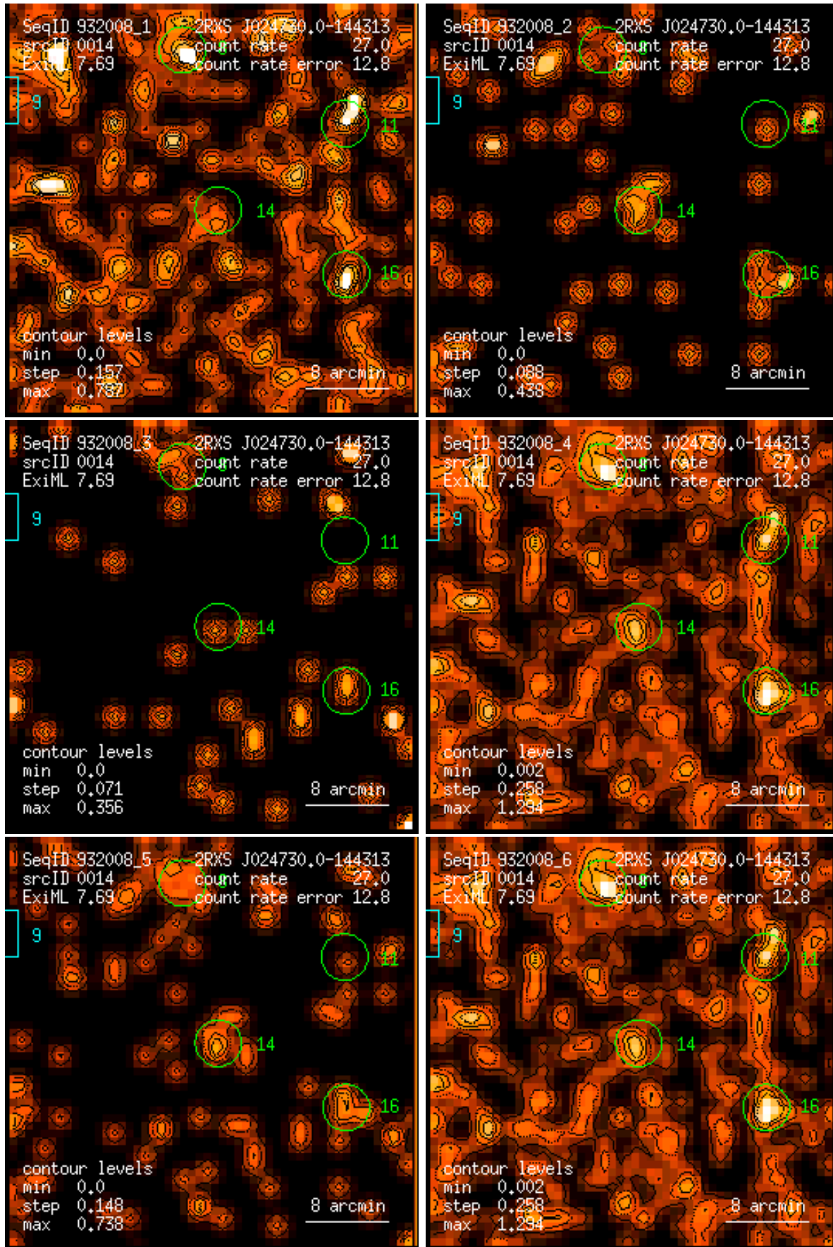
Figure 14: RASS 932008: detection 0014: band rate images, Gaussian filter: (1) PSPC channels 11 – 41, (2) 52 – 90, (3) 91 – 201, (4) 11 – 235, (5) 52 – 201, (6) 11 – 201. Broad band rates in counts/ks. Band rate contour levels in counts/ks/arcmin 2 .
