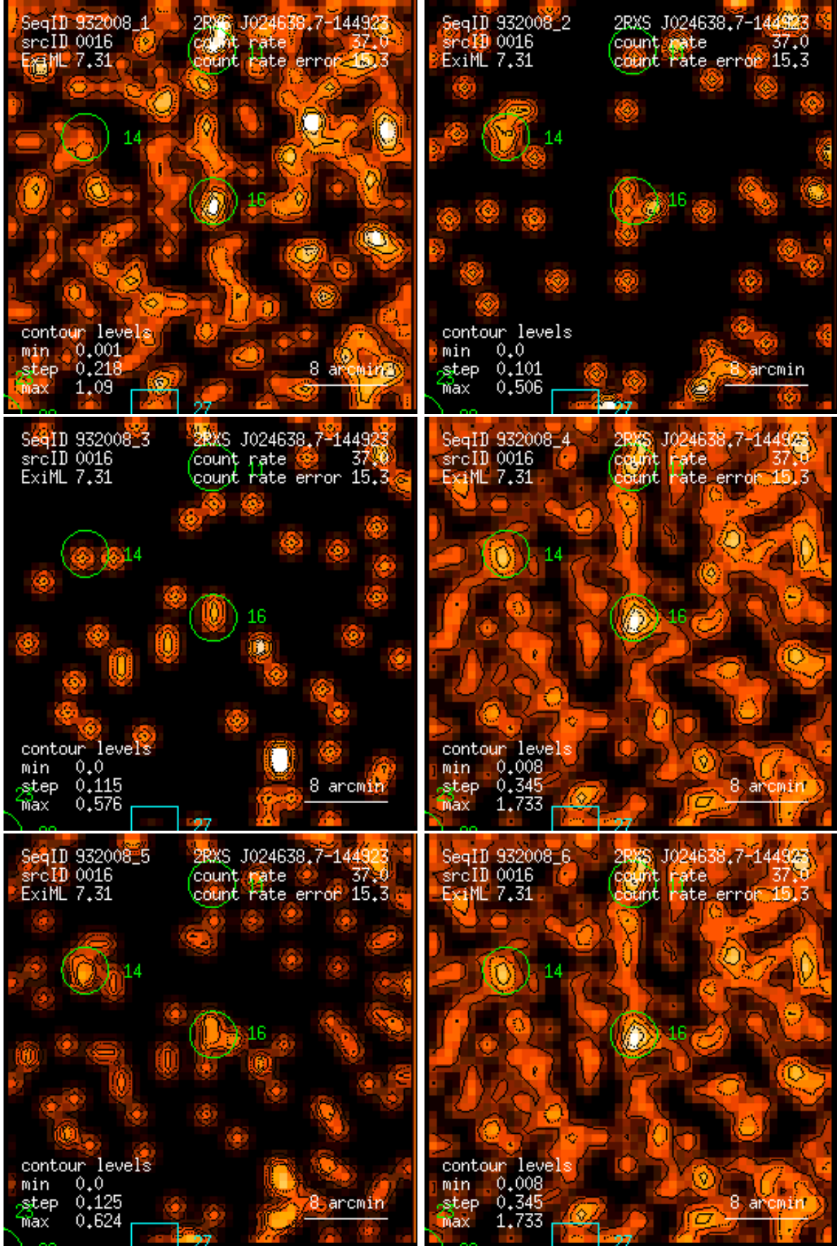
Figure 16: RASS 932008: detection 0016: band rate images, Gaussian filter: (1) PSPC channels 11 – 41, (2) 52 – 90, (3) 91 – 201, (4) 11 – 235, (5) 52 – 201, (6) 11 – 201. Broad band rates in counts/ks. Band rate contour levels in counts/ks/arcmin 2 .
