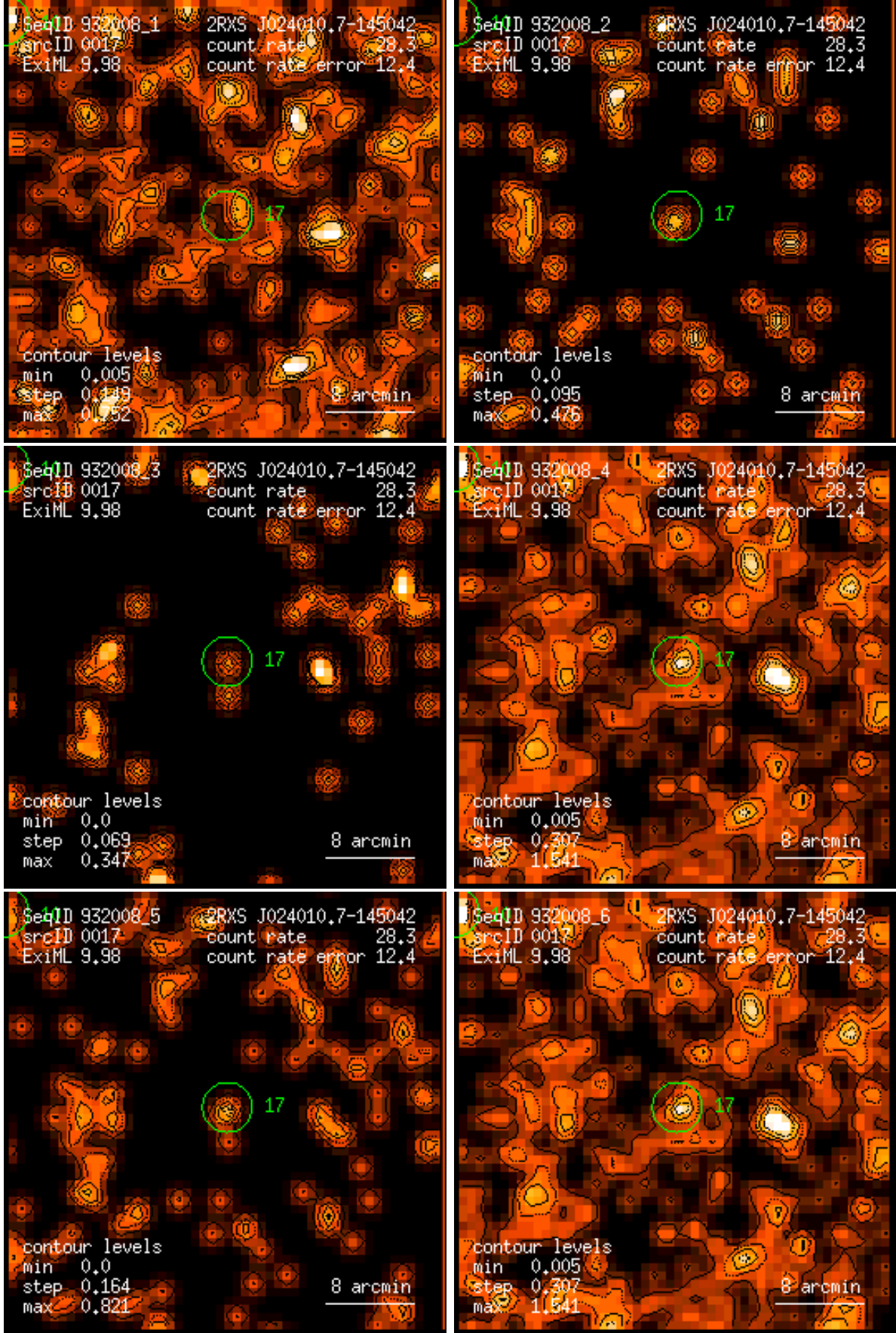
Figure 17: RASS 932008: detection 0017: band rate images, Gaussian filter: (1) PSPC channels 11 – 41, (2) 52 – 90, (3) 91 – 201, (4) 11 – 235, (5) 52 – 201, (6) 11 – 201. Broad band rates in counts/ks. Band rate contour levels in counts/ks/arcmin 2 .
