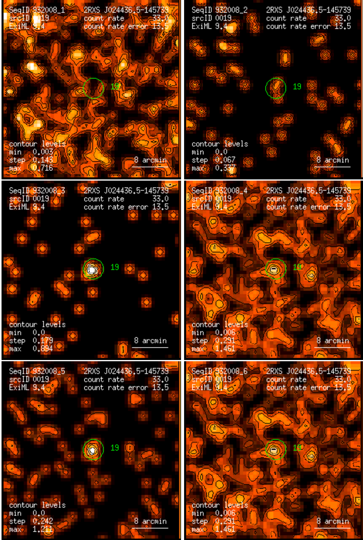
Figure 19: RASS 932008: detection 0019: band rate images, Gaussian filter: (1) PSPC channels 11 – 41, (2) 52 – 90, (3) 91 – 201, (4) 11 – 235, (5) 52 – 201, (6) 11 – 201. Broad band rates in counts/ks. Band rate contour levels in counts/ks/arcmin 2 .
