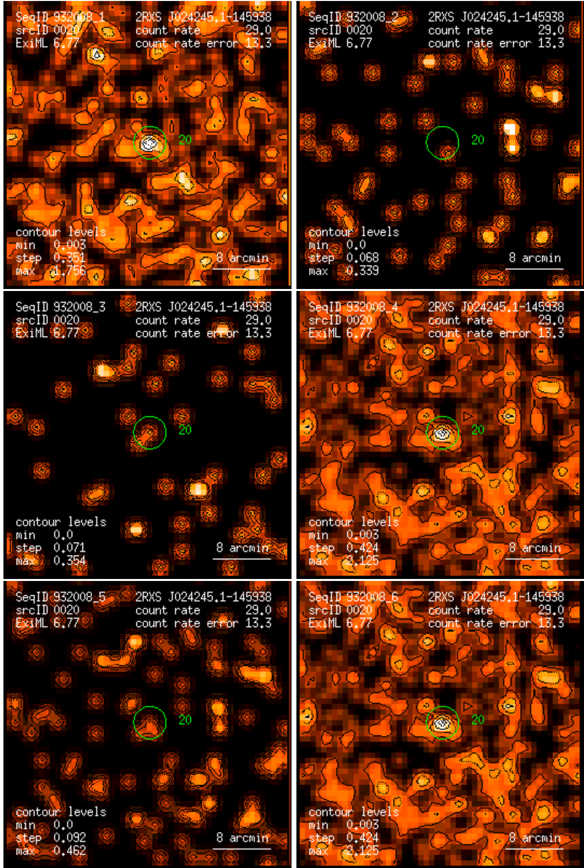
Figure 20: RASS 932008: detection 0020: band rate images, Gaussian filter: (1) PSPC channels 11 – 41, (2) 52 – 90, (3) 91 – 201, (4) 11 – 235, (5) 52 – 201, (6) 11 – 201. Broad band rates in counts/ks. Band rate contour levels in counts/ks/arcmin 2 .
