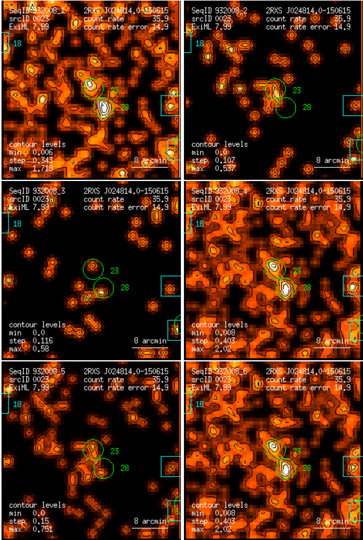
Figure 23: RASS 932008: detection 0023: band rate images, Gaussian filter: (1) PSPC channels 11 – 41, (2) 52 – 90, (3) 91 – 201, (4) 11 – 235, (5) 52 – 201, (6) 11 – 201. Broad band rates in counts/ks. Band rate contour levels in counts/ks/arcmin 2 .
