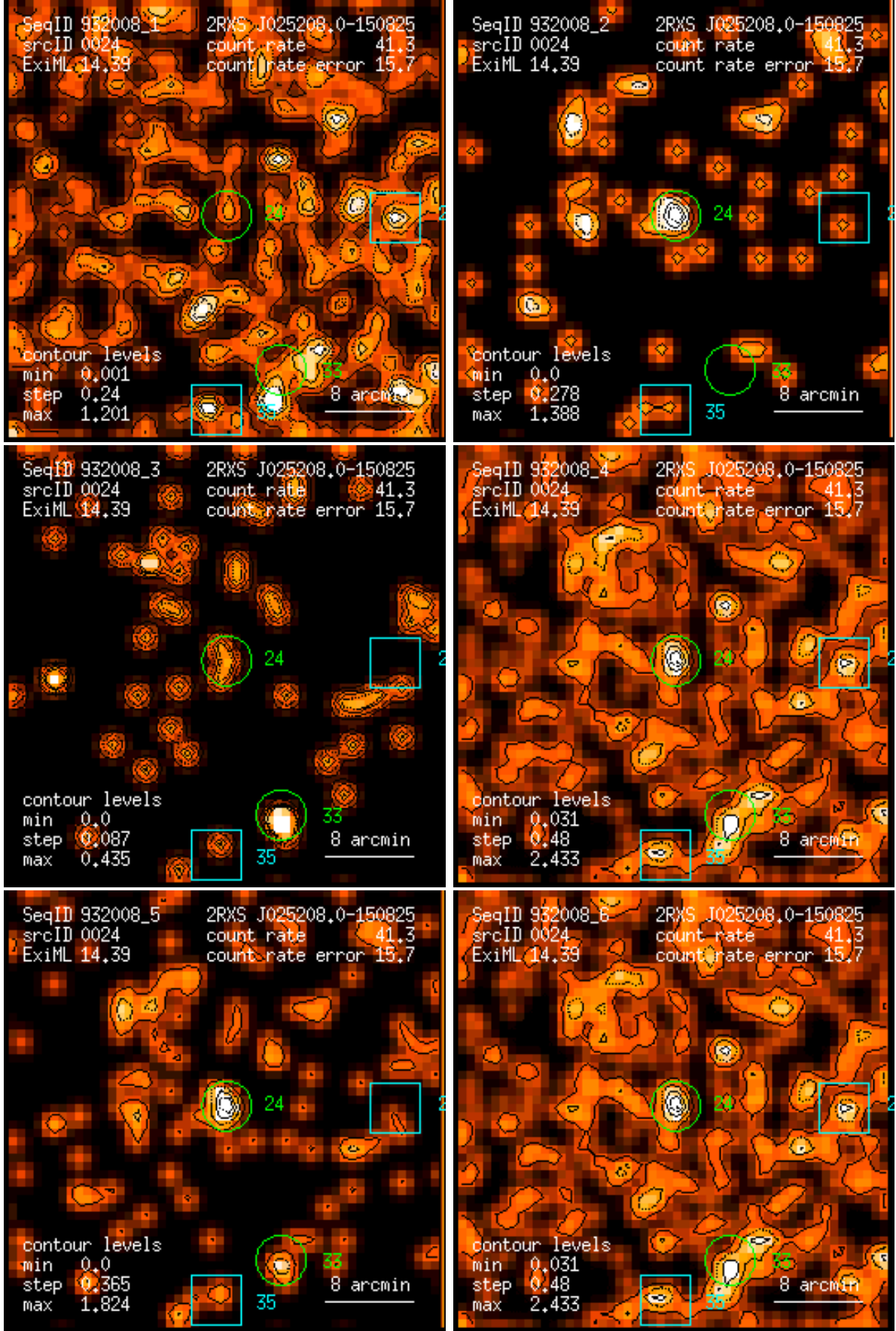
Figure 24: RASS 932008: detection 0024: band rate images, Gaussian filter: (1) PSPC channels 11 – 41, (2) 52 – 90, (3) 91 – 201, (4) 11 – 235, (5) 52 – 201, (6) 11 – 201. Broad band rates in counts/ks. Band rate contour levels in counts/ks/arcmin 2 .
