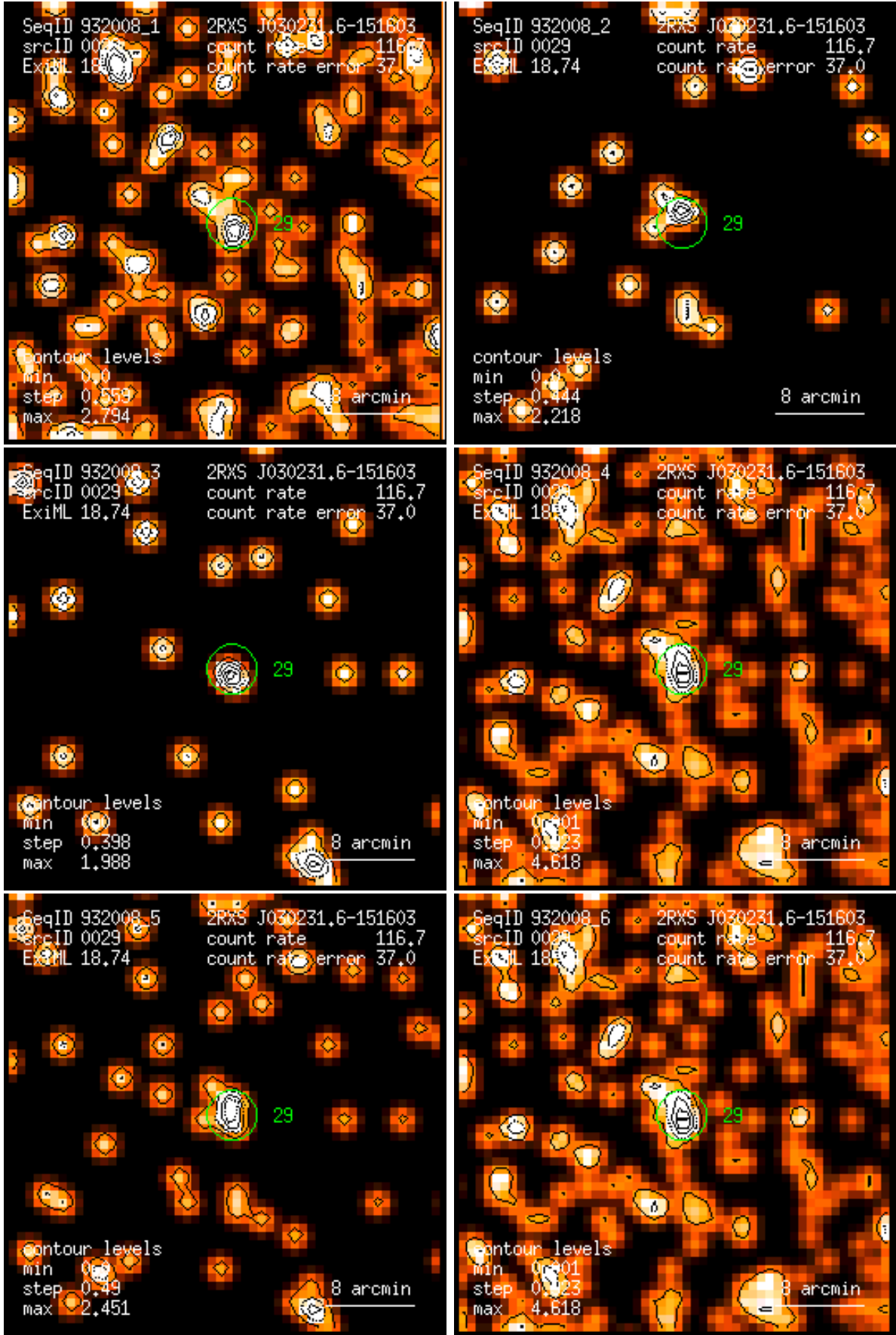
Figure 29: RASS 932008: detection 0029: band rate images, Gaussian filter: (1) PSPC channels 11 – 41, (2) 52 – 90, (3) 91 – 201, (4) 11 – 235, (5) 52 – 201, (6) 11 – 201. Broad band rates in counts/ks. Band rate contour levels in counts/ks/arcmin 2 .
