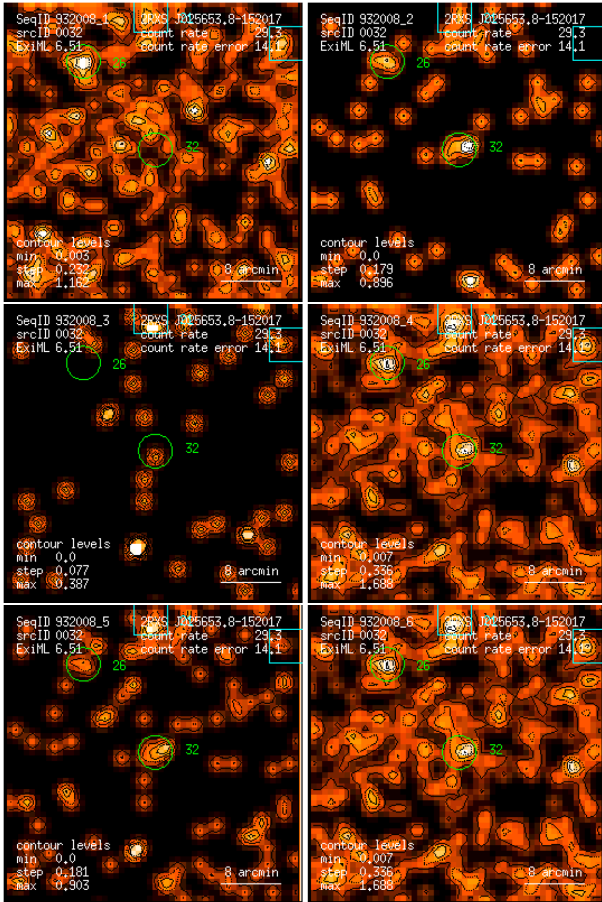
Figure 32: RASS 932008: detection 0032: band rate images, Gaussian filter: (1) PSPC channels 11 – 41, (2) 52 – 90, (3) 91 – 201, (4) 11 – 235, (5) 52 – 201, (6) 11 – 201. Broad band rates in counts/ks. Band rate contour levels in counts/ks/arcmin 2 .
