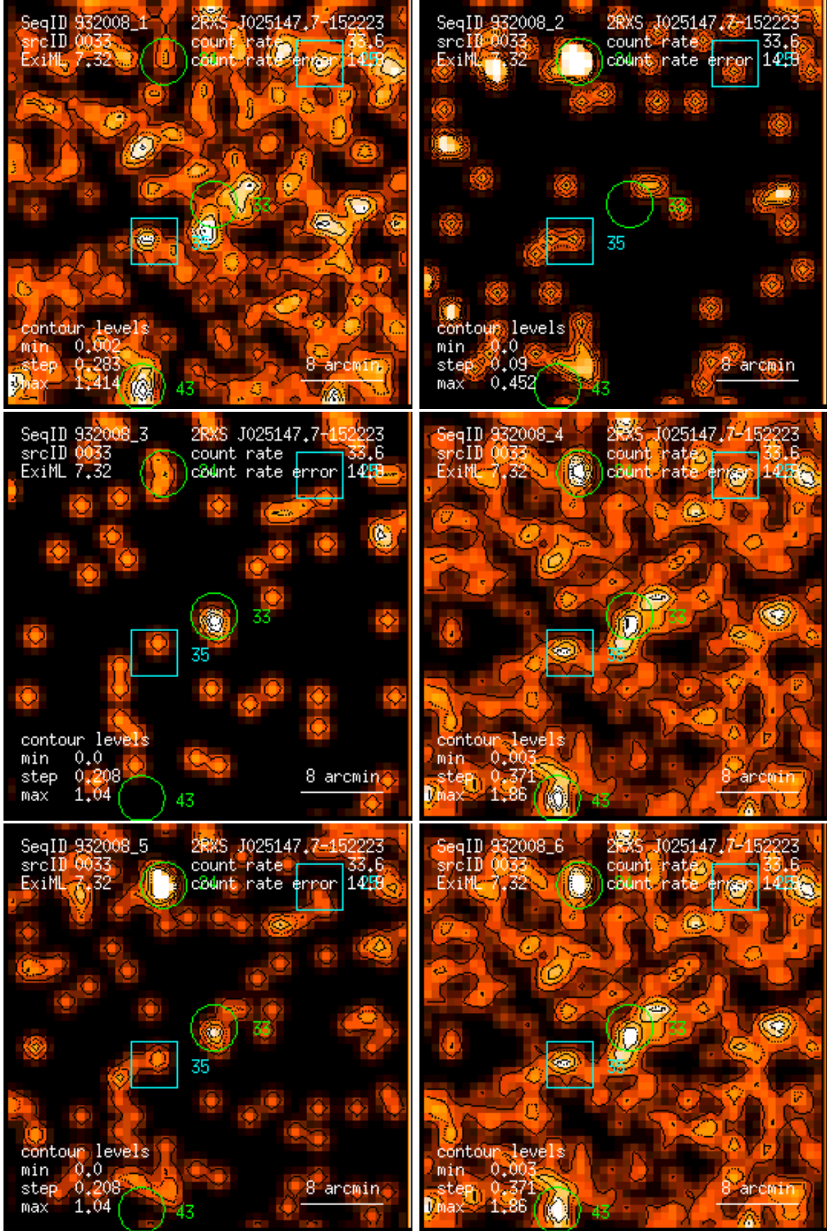
Figure 33: RASS 932008: detection 0033: band rate images, Gaussian filter: (1) PSPC channels 11 – 41, (2) 52 – 90, (3) 91 – 201, (4) 11 – 235, (5) 52 – 201, (6) 11 – 201. Broad band rates in counts/ks. Band rate contour levels in counts/ks/arcmin 2 .
