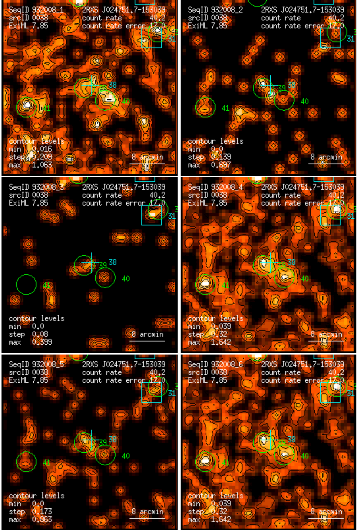
Figure 38: RASS 932008: detection 0038: band rate images, Gaussian filter: (1) PSPC channels 11 – 41, (2) 52 – 90, (3) 91 – 201, (4) 11 – 235, (5) 52 – 201, (6) 11 – 201. Broad band rates in counts/ks. Band rate contour levels in counts/ks/arcmin 2 .
