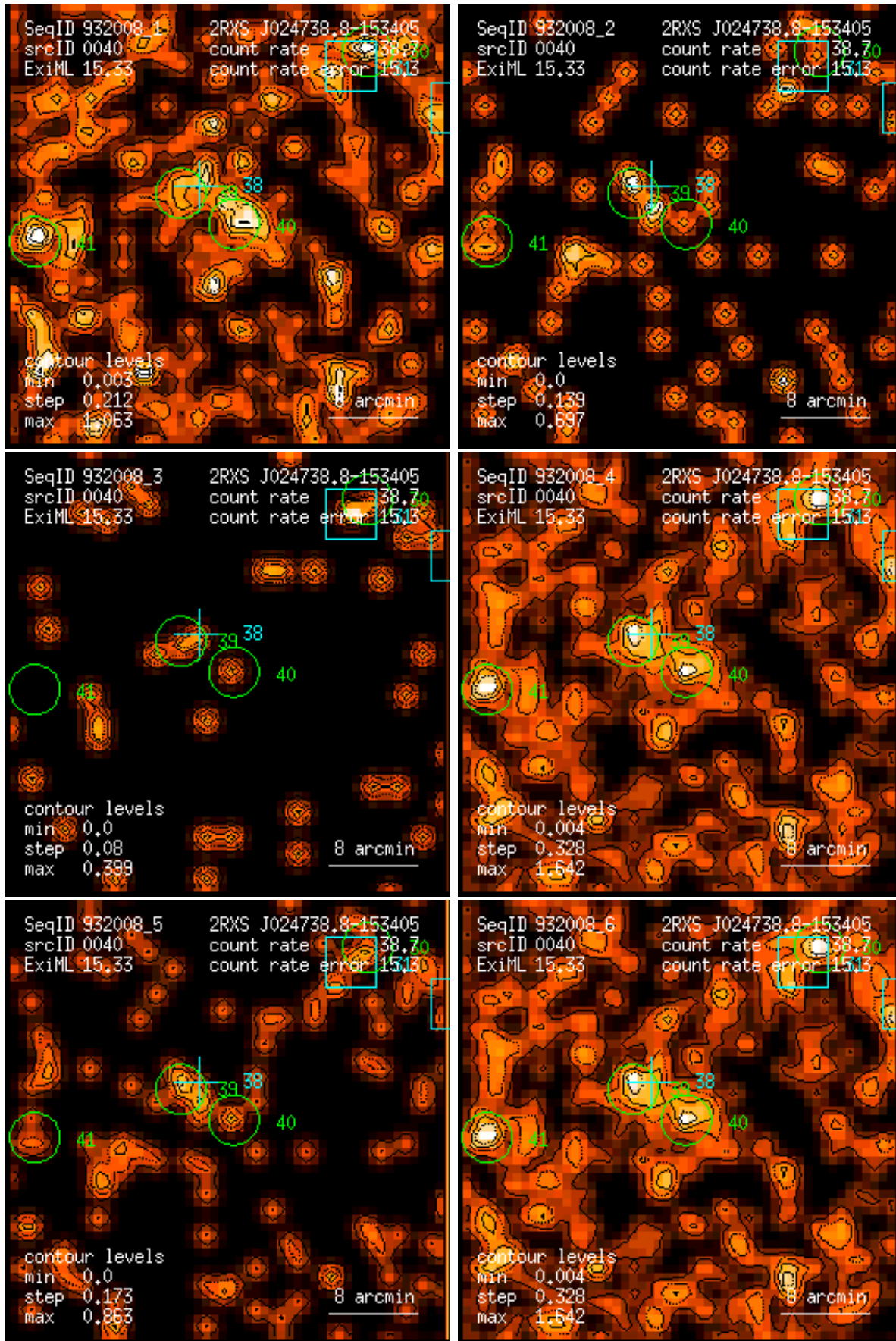
Figure 40: RASS 932008: detection 0040: band rate images, Gaussian filter: (1) PSPC channels 11 – 41, (2) 52 – 90, (3) 91 – 201, (4) 11 – 235, (5) 52 – 201, (6) 11 – 201. Broad band rates in counts/ks. Band rate contour levels in counts/ks/arcmin 2 .
