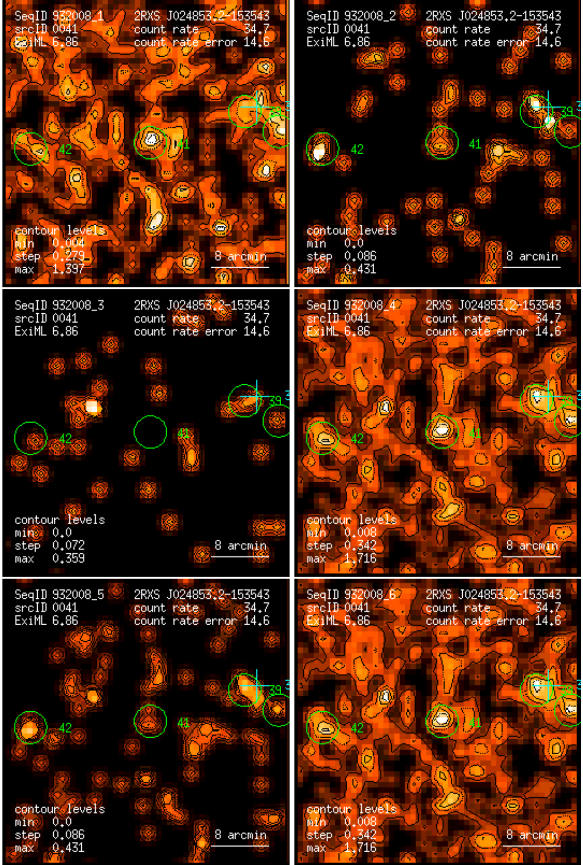
Figure 41: RASS 932008: detection 0041: band rate images, Gaussian filter: (1) PSPC channels 11 – 41, (2) 52 – 90, (3) 91 – 201, (4) 11 – 235, (5) 52 – 201, (6) 11 – 201. Broad band rates in counts/ks. Band rate contour levels in counts/ks/arcmin 2 .
