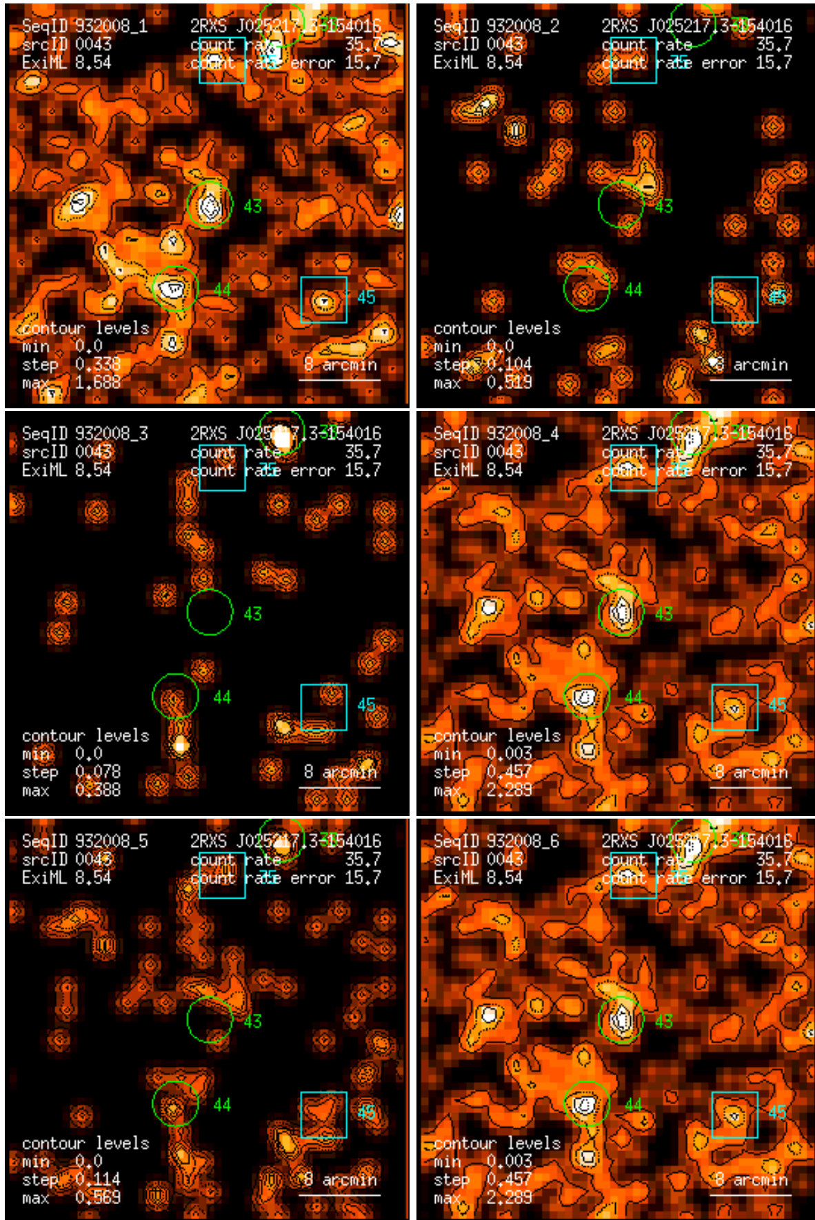
Figure 43: RASS 932008: detection 0043: band rate images, Gaussian filter: (1) PSPC channels 11 – 41, (2) 52 – 90, (3) 91 – 201, (4) 11 – 235, (5) 52 – 201, (6) 11 – 201. Broad band rates in counts/ks. Band rate contour levels in counts/ks/arcmin 2 .
