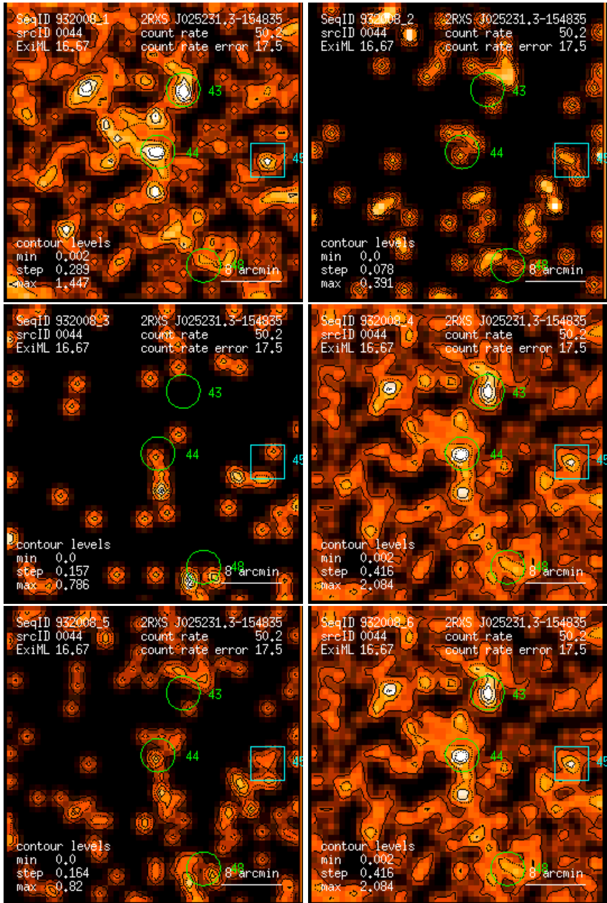
Figure 44: RASS 932008: detection 0044: band rate images, Gaussian filter: (1) PSPC channels 11 – 41, (2) 52 – 90, (3) 91 – 201, (4) 11 – 235, (5) 52 – 201, (6) 11 – 201. Broad band rates in counts/ks. Band rate contour levels in counts/ks/arcmin 2 .
