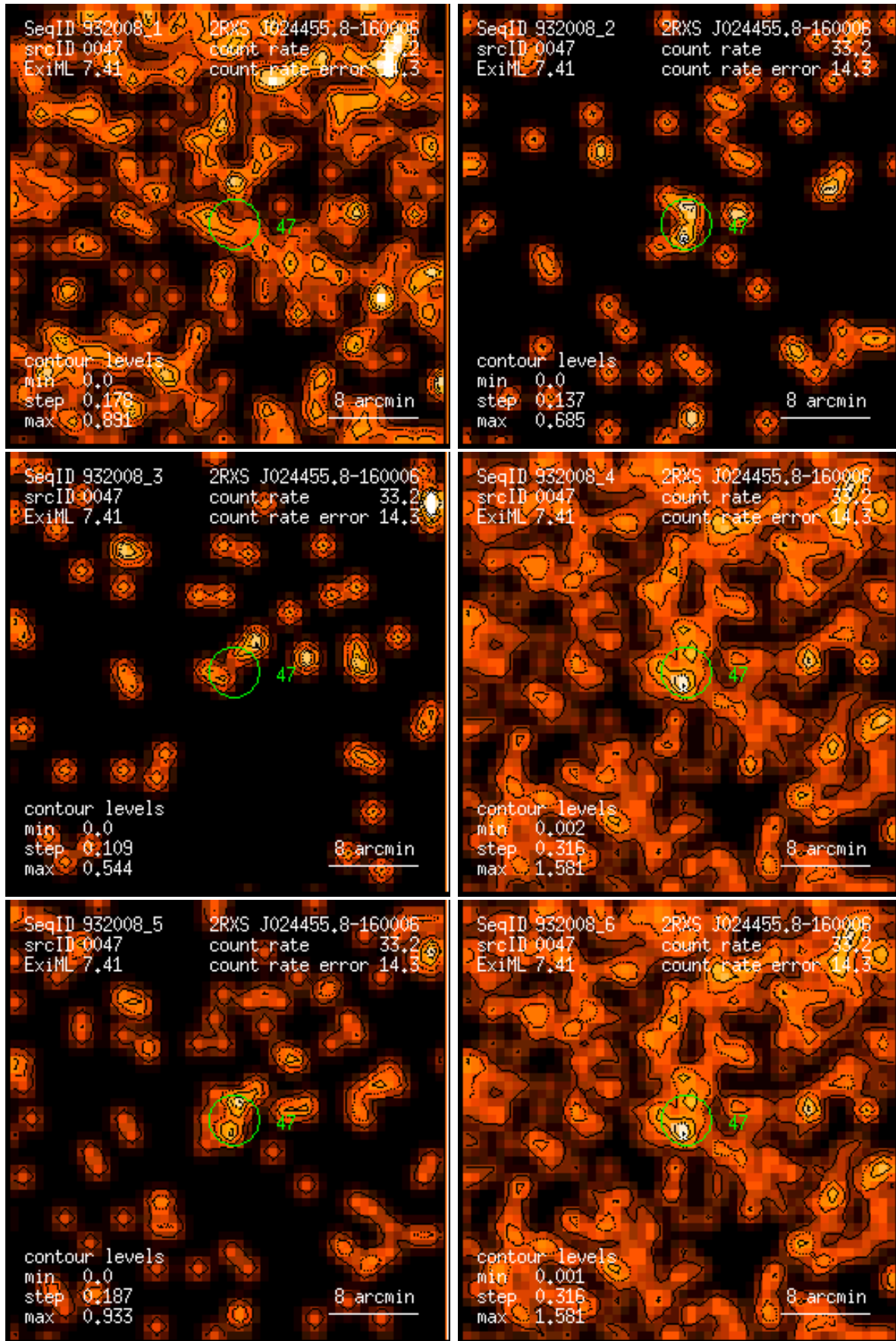
Figure 47: RASS 932008: detection 0047: band rate images, Gaussian filter: (1) PSPC channels 11 – 41, (2) 52 – 90, (3) 91 – 201, (4) 11 – 235, (5) 52 – 201, (6) 11 – 201. Broad band rates in counts/ks. Band rate contour levels in counts/ks/arcmin 2 .
