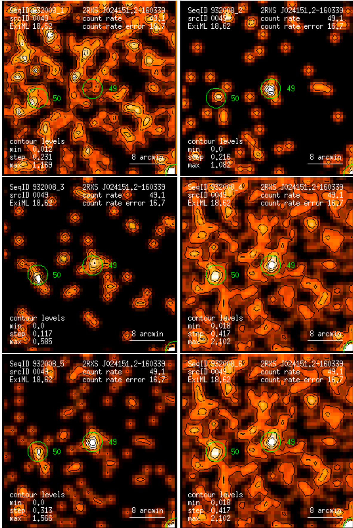
Figure 49: RASS 932008: detection 0049: band rate images, Gaussian filter: (1) PSPC channels 11 – 41, (2) 52 – 90, (3) 91 – 201, (4) 11 – 235, (5) 52 – 201, (6) 11 – 201. Broad band rates in counts/ks. Band rate contour levels in counts/ks/arcmin 2 .
