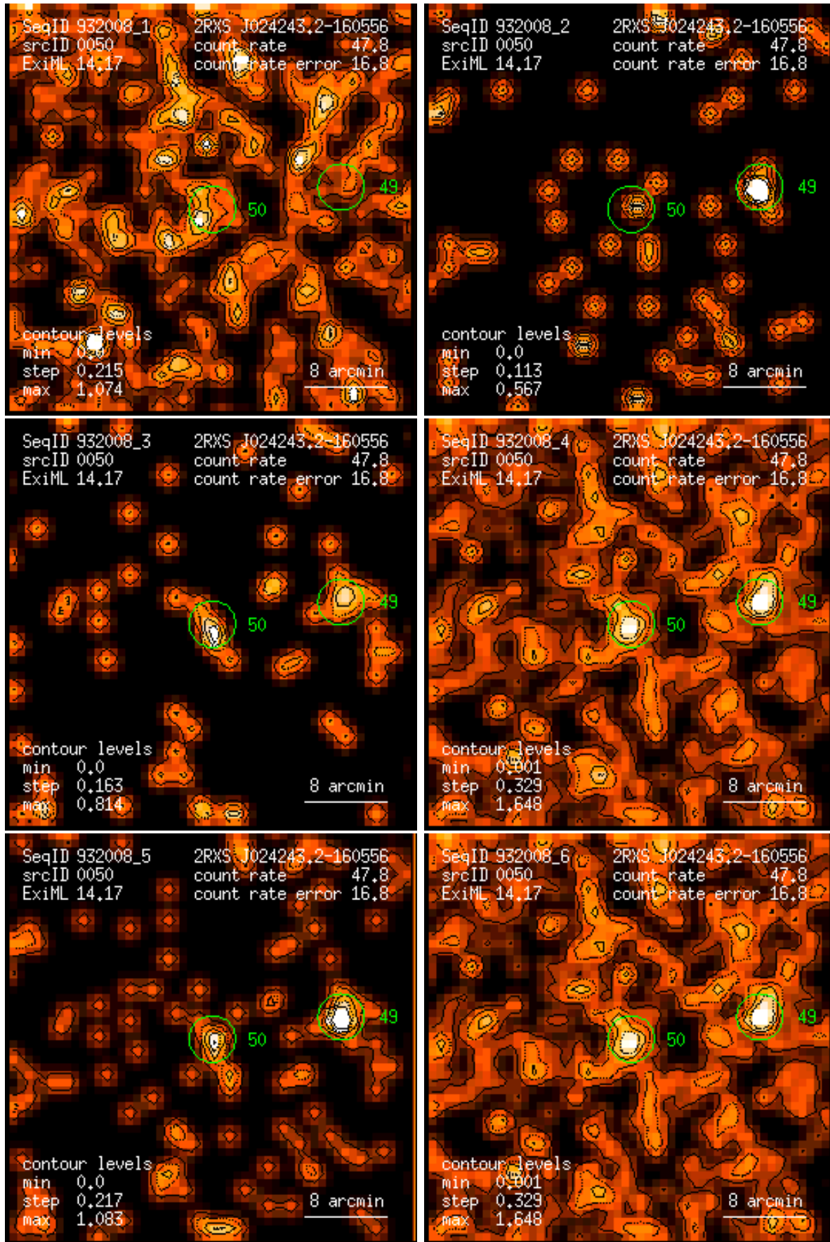
Figure 50: RASS 932008: detection 0050: band rate images, Gaussian filter: (1) PSPC channels 11 – 41, (2) 52 – 90, (3) 91 – 201, (4) 11 – 235, (5) 52 – 201, (6) 11 – 201. Broad band rates in counts/ks. Band rate contour levels in counts/ks/arcmin 2 .
