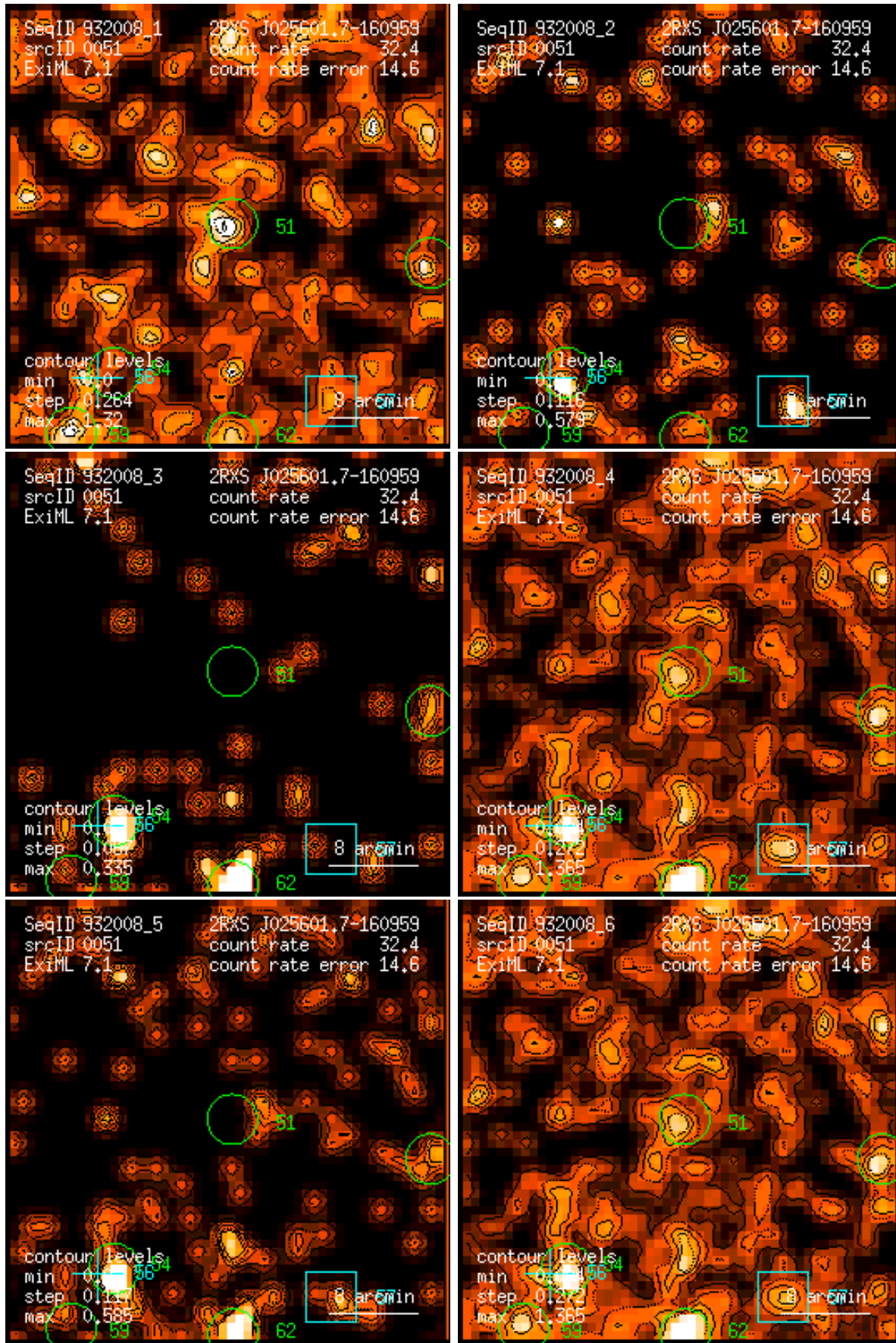
Figure 51: RASS 932008: detection 0051: band rate images, Gaussian filter: (1) PSPC channels 11 – 41, (2) 52 – 90, (3) 91 – 201, (4) 11 – 235, (5) 52 – 201, (6) 11 – 201. Broad band rates in counts/ks. Band rate contour levels in counts/ks/arcmin 2 .
