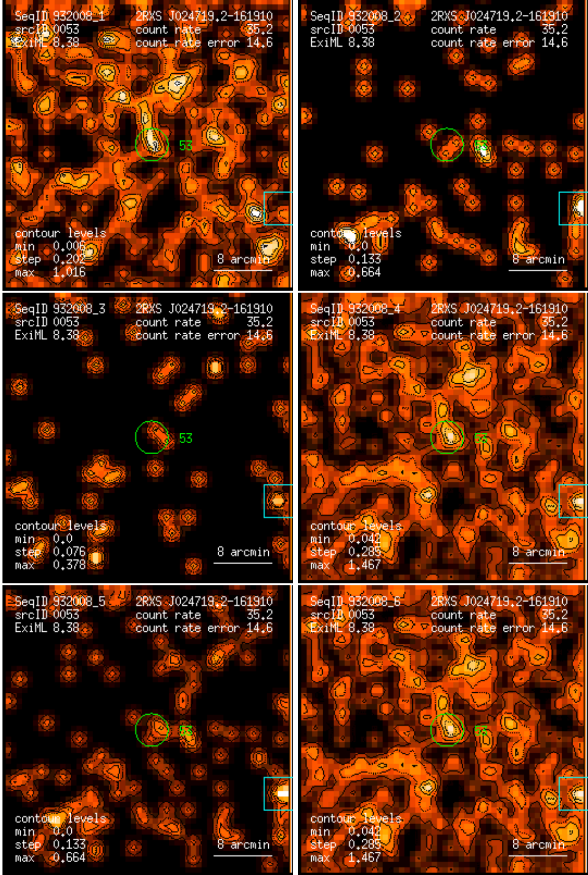
Figure 53: RASS 932008: detection 0053: band rate images, Gaussian filter: (1) PSPC channels 11 – 41, (2) 52 – 90, (3) 91 – 201, (4) 11 – 235, (5) 52 – 201, (6) 11 – 201. Broad band rates in counts/ks. Band rate contour levels in counts/ks/arcmin 2 .
