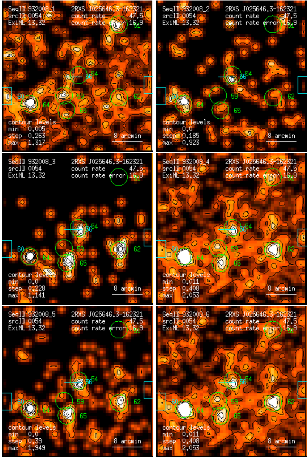
Figure 54: RASS 932008: detection 0054: band rate images, Gaussian filter: (1) PSPC channels 11 – 41, (2) 52 – 90, (3) 91 – 201, (4) 11 – 235, (5) 52 – 201, (6) 11 – 201. Broad band rates in counts/ks. Band rate contour levels in counts/ks/arcmin 2 .
